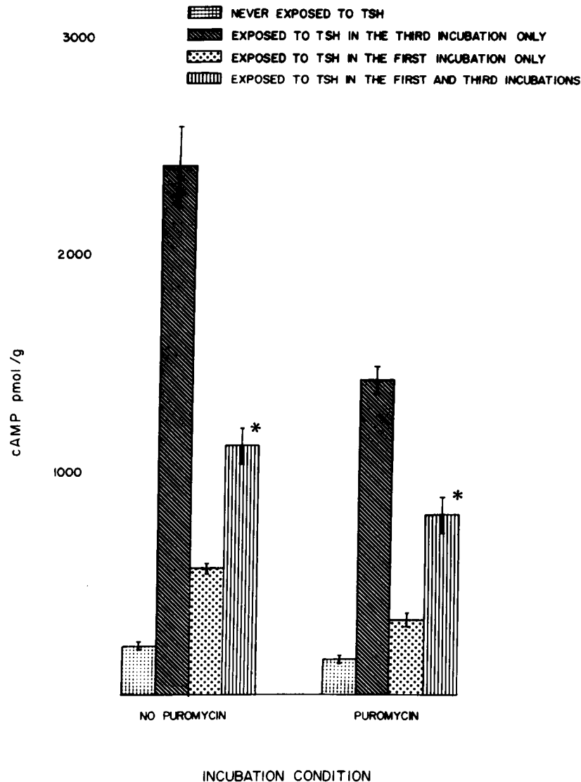
FIGURE 3 Failure of puromycin to modify refractoriness to TSH. Beef thyroid slices were incubated with or without puromycin (150 \mu\text{g}/\text{ml} ) for 15 min before commencing the first incubation which was 120 min. All subsequent incubation media for slices initially exposed to puromycin also contained this substance. The second incubation was for 60 min and the third was for 20 min. The values represent the mean \pm SEM of triplicate slices. The TSH concentration was 50 mU/ml.
