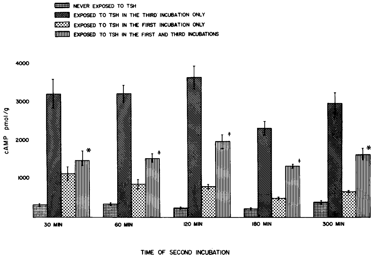
FIGURE 2 Effect of length of the second incubation on the subsequent cyclic AMP response to TSH. The first incubation was 120 min and the second incubation varied as indicated. The third incubation was 20 min. Different beef thyroid glands were used for each time. The values are the mean \pm SEM of triplicate slices. The TSH concentration was 50 mU/ml. * P < 0.02 when compared to slices exposed to TSH in the third incubation only. † P < 0.01 when compared to slices exposed to TSH in the third incubation only.
