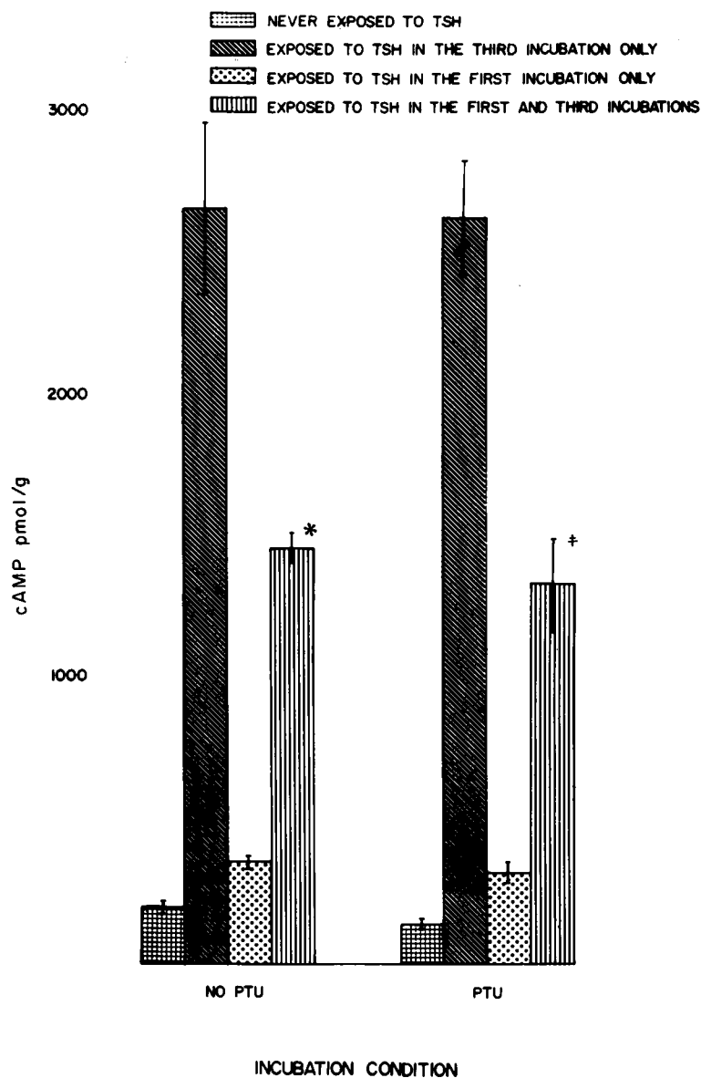
FIGURE 4 Failure of propylthiouracil (PTU) to abolish TSH refractoriness. Beef thyroid slices were incubated with or without (3 mM) PTU for 15 min before commencing the first incubation which was for 120 min. All subsequent incubation media for slices initially exposed to PTU also contained this substance. The second incubation was for 180 min and third for 20 min. The values represent the mean \pm SEM of triplicate slices. The TSH concentration was 50 mU/ml.
