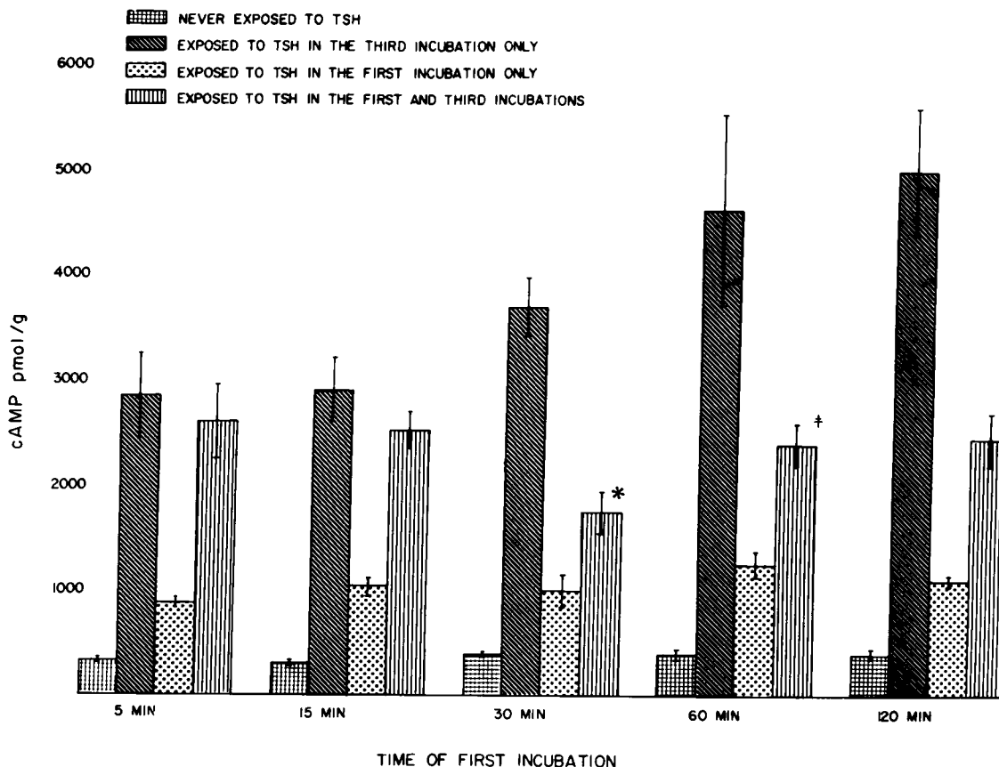
FIGURE 1 Effect of length of the first incubation on the subsequent cyclic AMP response to TSH. The second incubation was 120 min and the third incubation was 20 min. A single beef thyroid was used for the entire experiment. The values are the mean \pm SEM of triplicate slices. The TSH concentration was 50 mU/ml.
