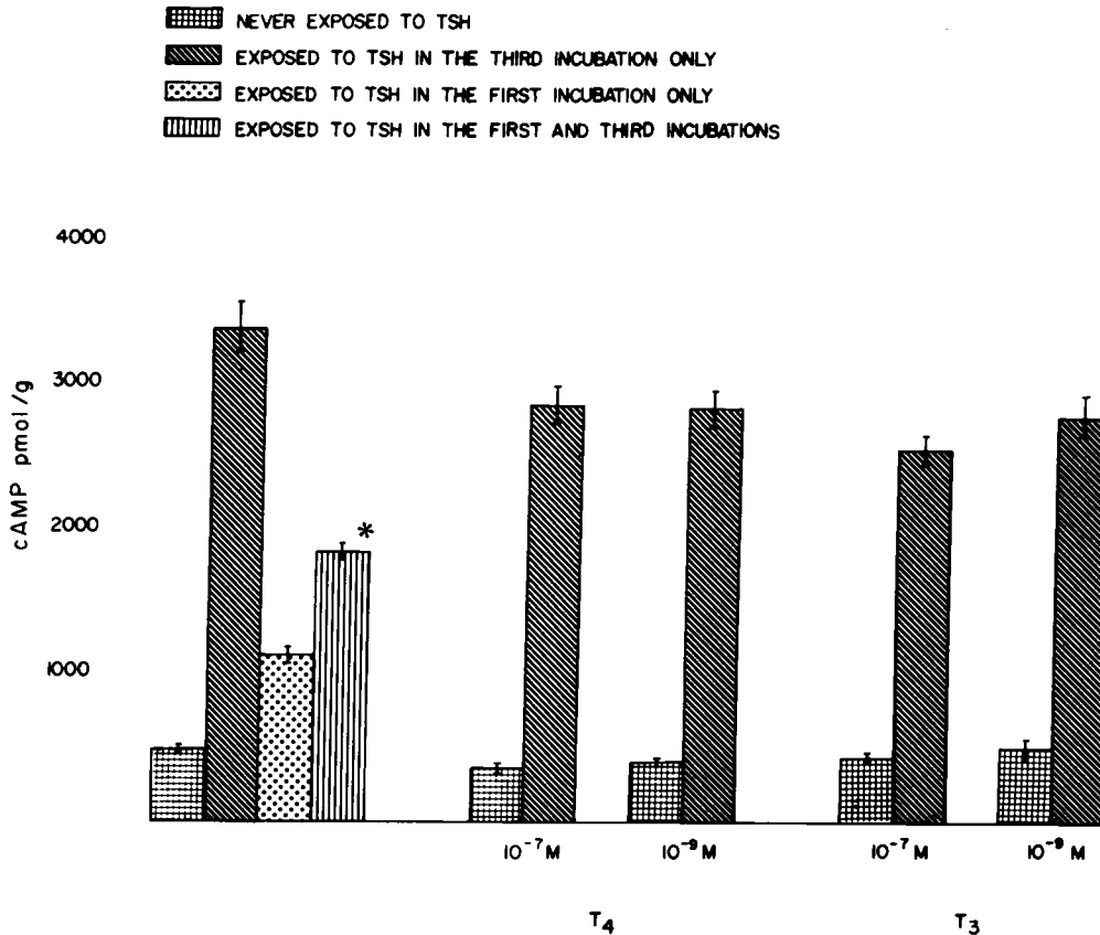
FIGURE 5 Failure of T 4 and T 3 to induce refractoriness to TSH. Beef thyroid slices were incubated with or without 0.1 \mu M or 1 nM T 4 or T 3 during all three incubations. The first and second incubations were for 120 min each while the third incubation was for 20 min. The values are the mean \pm SEM of triplicate slices. The TSH concentration was 50 mU/ml. In the presence and absence of 0.1 \mu M T 3 , the effect of TSH added in the third incubation only was significantly less ( P < 0.05 ) in the former slices.
