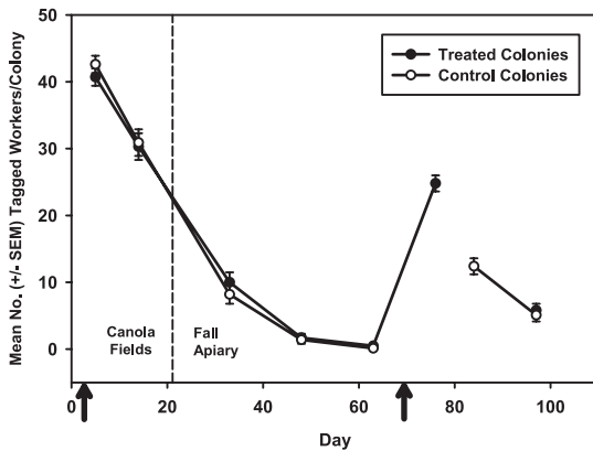
Fig. 4. Mean \pm SEM honey bee worker longevity in colonies in clothianidin-treated and control canola fields. Fifty workers tagged with colored/numbered thoracic tags were added to each colony (denoted by arrows on x-axis) on Day 4 and again on Day 70. Colonies were in canola fields the first 21 d of the experiment and thereafter moved to a fall apiary until 130 d from initial exposure to canola. Tagged workers in each colony were counted approximately every 14 d except on Day 76/77 and Day 84 for control and clothianidin-treated colonies, respectively.
