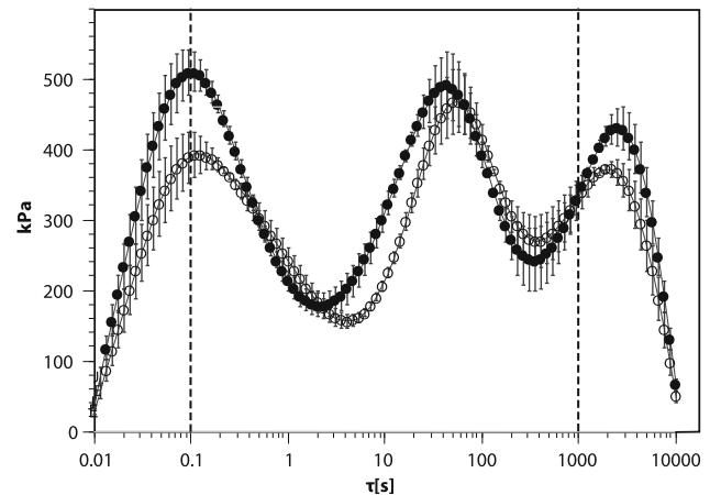
Fig. 7 Relaxation spectra of wild type ( open symbols ) and PAT31 ( closed symbols ). Dashed lines indicate the reliable range; meaning of error bars is given in Hansen et al. (2011). \tau time in s
