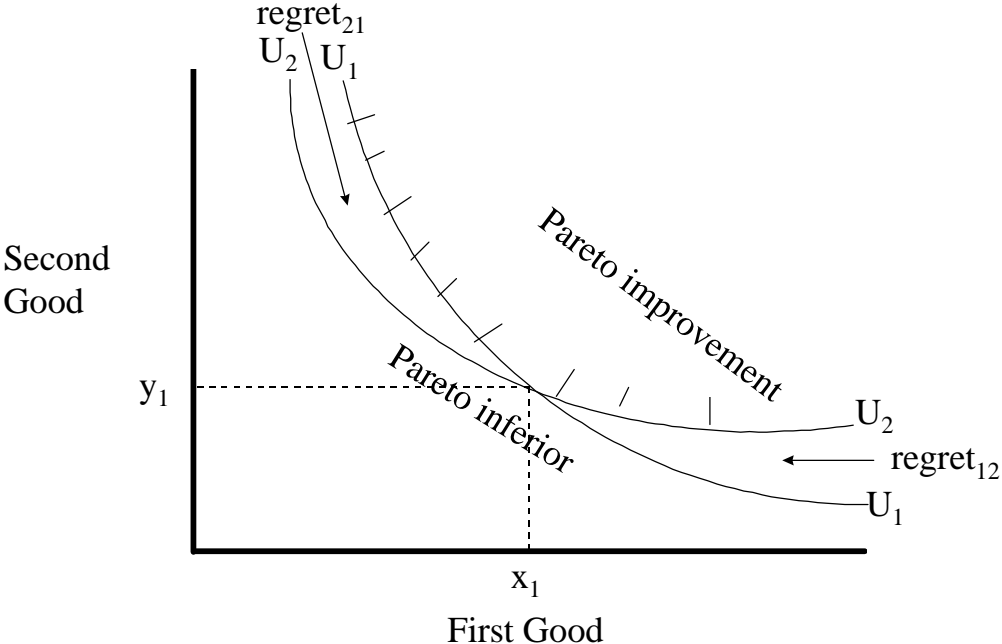
Figure 5: Pareto Improvement
