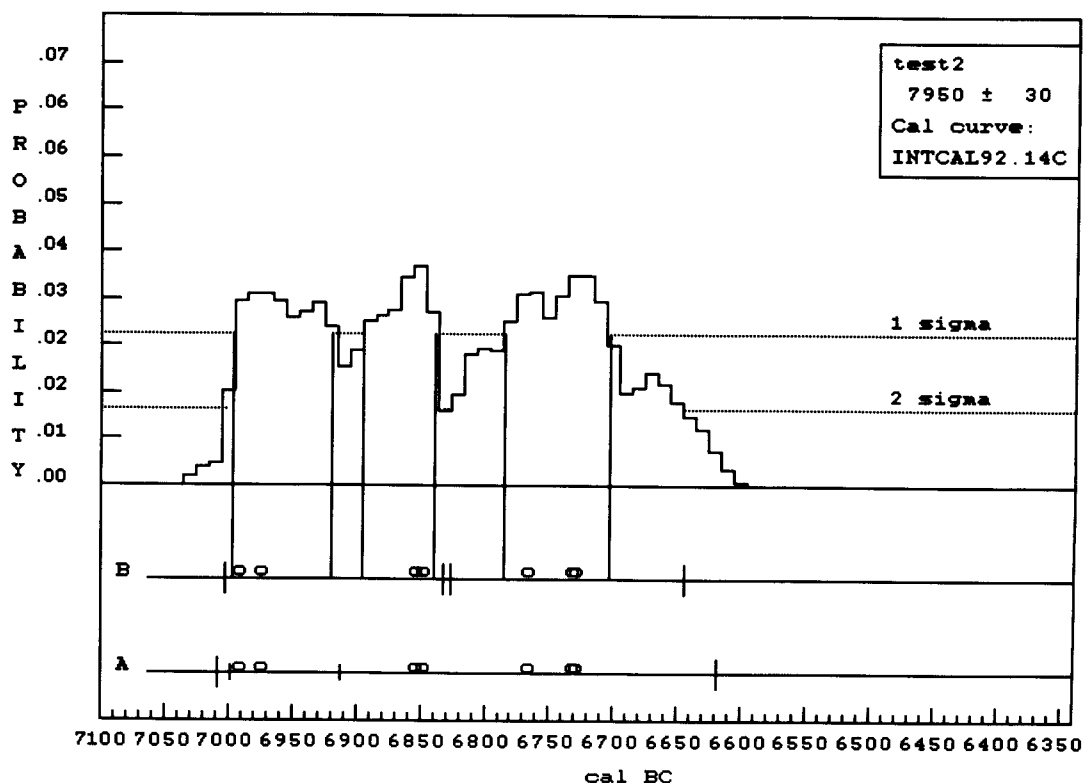
Fig. 7. The probability distribution from CALIB 3.0 for a test sample plotted as a histogram with Methods A and B cal age ranges marked by vertical lines (see Fig. 5) and cal ages represented by circles
