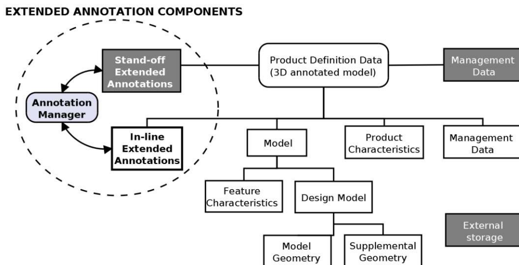
Fig. 3. Extended Annotation Model (Adapted From [29])
