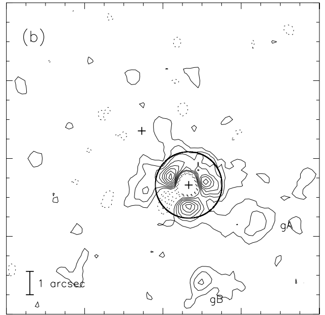
Figure 4. U -band contour plot of the same field as in Fig. 2. (a) final combined frame showing the two quasars. The contour levels are -9, -6, -3, 3, 6, \dots \times 1\sigma of the sky noise, with the dotted contours being negative. (b) Final combined frame (same contour levels as above) after subtraction of the quasar images.
