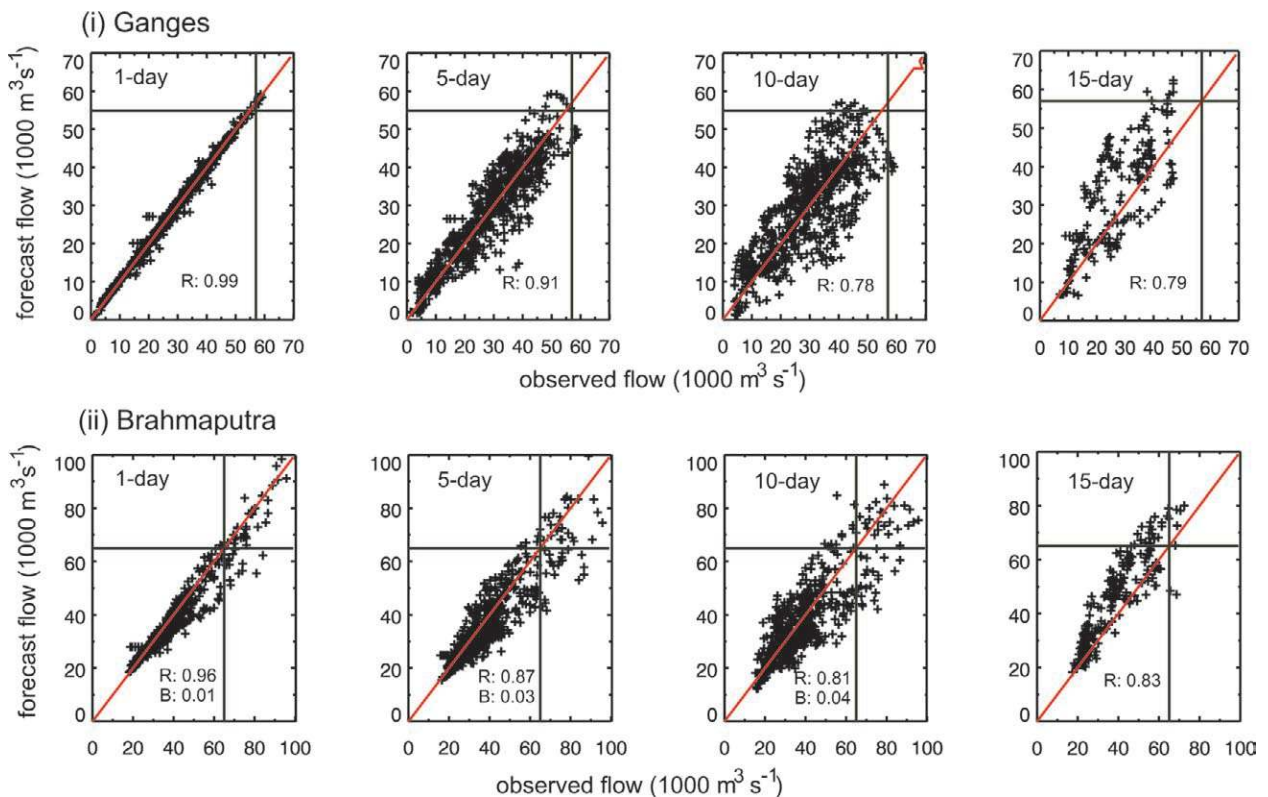
FIG. 13. Verification statistics for the (i) Ganges and (ii) Brahmaputra. Figures compare the ensemble mean of the discharge forecasts with the 5-, 10-, and 15-days observed discharge. Correlations (R) and the Brier score (B) are also plotted. Statistics for the 15-day forecasts refer only to 2008 and 2009.
