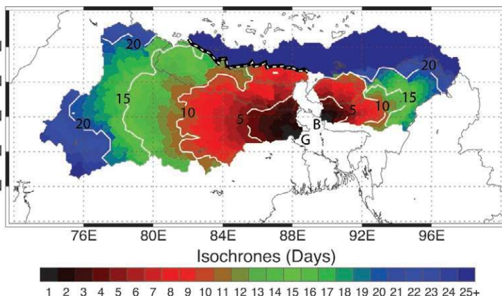
FIG. 5. Isochrone (days) for the Brahmaputra and Ganges basins. The contours estimate the time taken for water at a particular location in the basin to pass to Bahadurabad or Hardinge Bridge, the staging stations shown in Fig. 1c. Isochrone were constructed using a flow routing algorithm and digital elevation data. The separation of the two basins is shown as a thick dashed white line. The 5-, 10-, 15-, and 20-day isochrones are shown as solid white lines.
