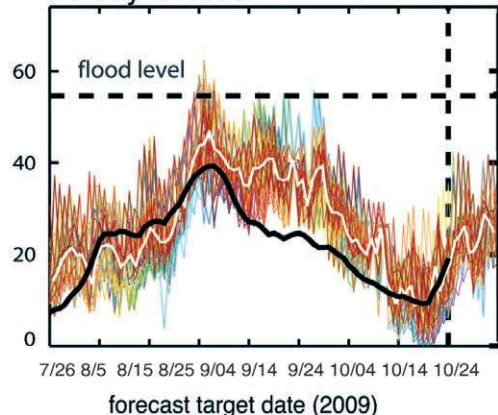
FIG. 12. As in Fig. 9, but for 2009 for the (a) Brahmaputra and (b) Ganges forecasts for 2009.
