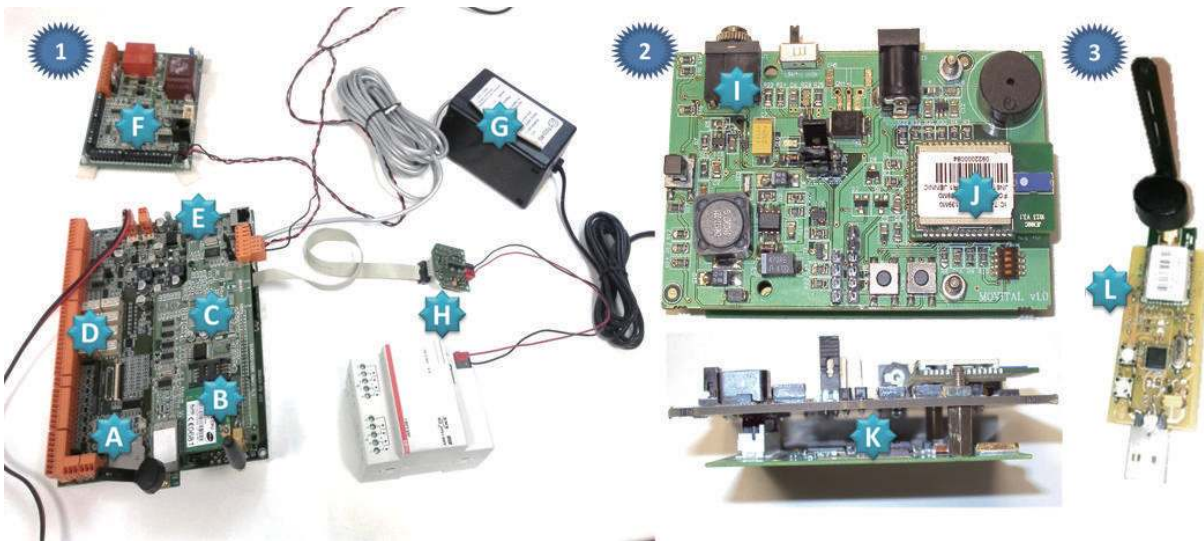
Fig. 3. (1) Multiprotocol card with 6LoWPAN (A), GPRS (B), Bluetooth (C), native interfaces (D), Ethernet (E), CAN (F), X10 (G), and KNX (H). (2) Movital adapter with native interfaces (I), 6LoWPAN (J) and RFID (K). (3) 6LoWPAN Bridge based on USB (L) from 6LoWPAN to Ethernet.
