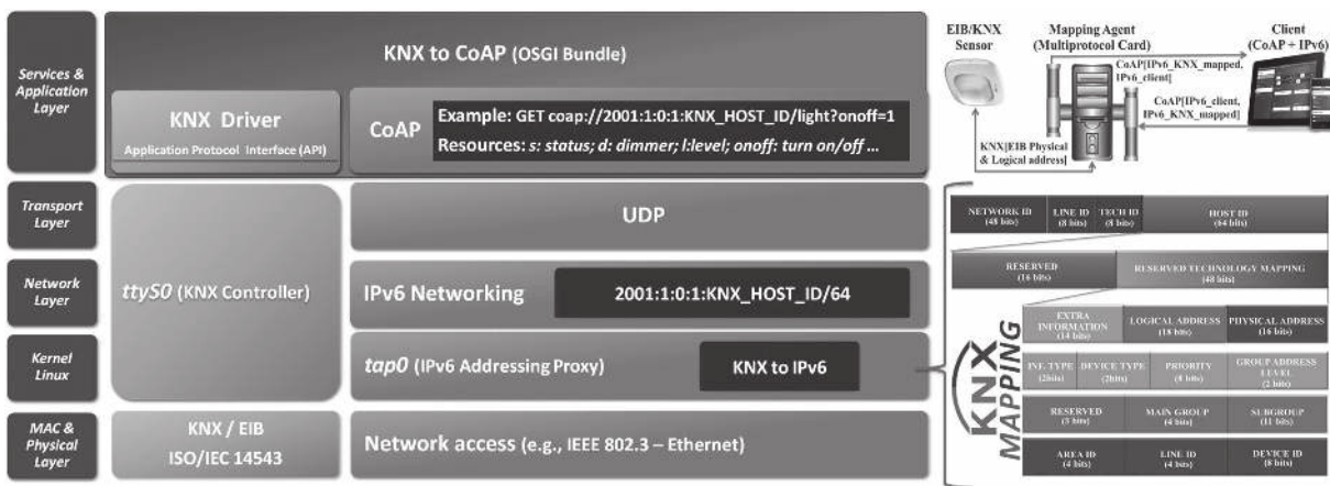
Fig. 5. Left: Internet integration stack instance for KNX integration. Right: KNX mapping from native addressing to IPv6 and translation process.
