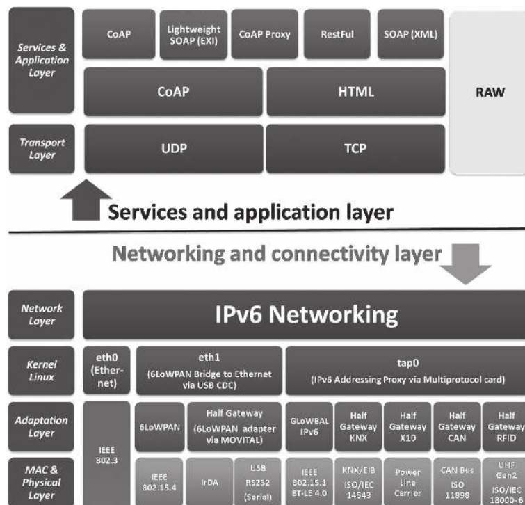
Fig. 1. Integration of Things in IPv6 stack.
