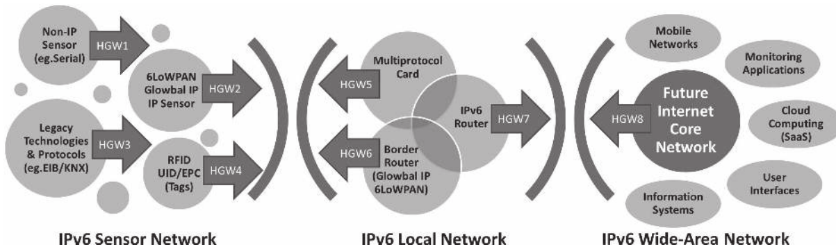
Fig. 2. Schematic of the topology envisaged to integrate in IPv6 through half-gateways from the sensor level to the Future Internet Core Network.
