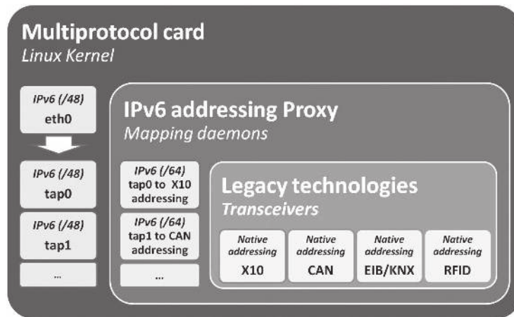
Fig. 4. IPv6 addressing proxy integration in the multiprotocol card.
