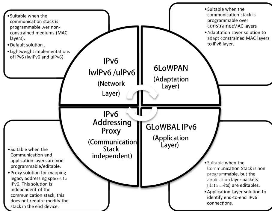
Fig. 6. Classification of the presented solutions in function of the communication layer upgraded.
