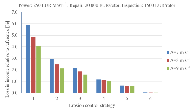
Figure 21. Loss of income due to erosion, inspection and repair. Energy: 250 EUR MWh -1 . Repair: 20 000 EUR rotor -1 . Inspection: 1500 EUR rotor -1 .
