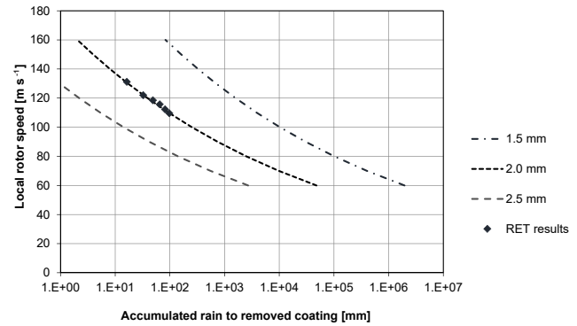
Figure 6. Expected accumulated rain to remove coating as a function of rotor speed for droplet diameters of 1.5, 2.0 and 2.5 mm.
