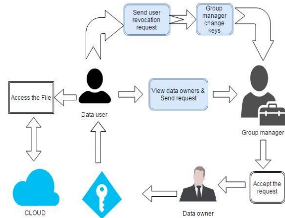
Figure 2. CP-ABE
