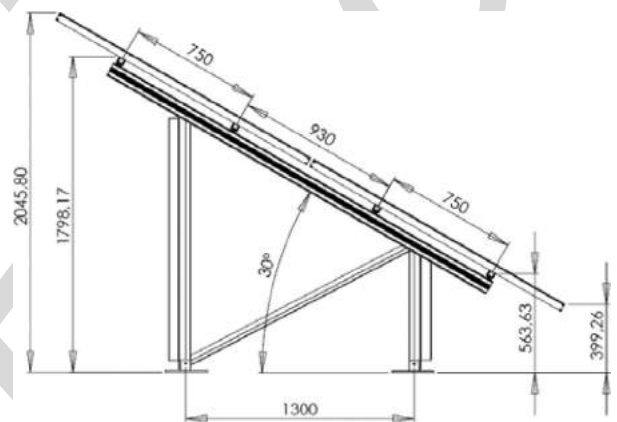
Fig. 10. Design dimensions (mm) of the PV structural base—side view.
