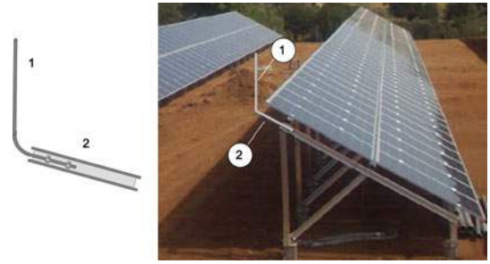
Fig. 2. Nonisolated L.P.S in PV applications. (1) Aluminum air termination rod. (2) Connection clamp.
