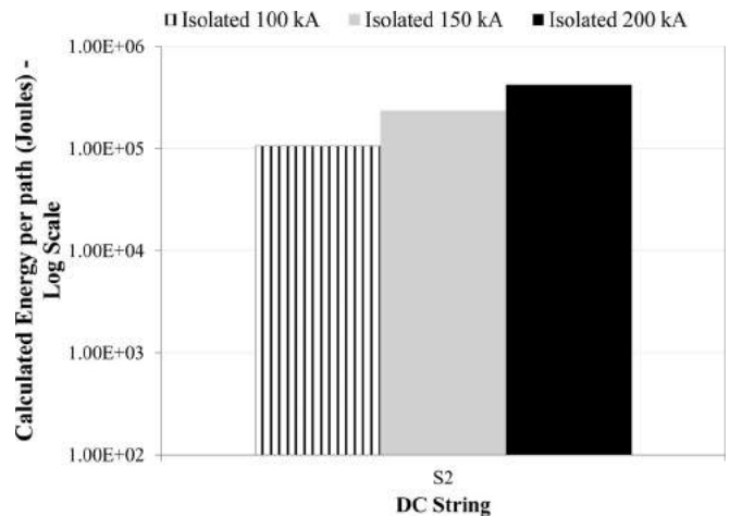
Fig. 16. Maximum dissipated energy across the 150-kW solar park with non-isolated L.P.S for different L.P.Cs.
