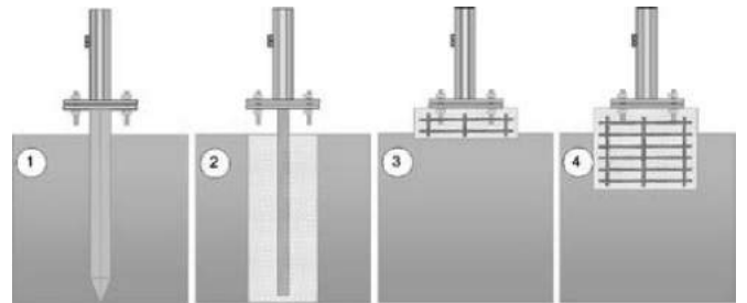
Fig. 3. Type of foundation for an earthing system of the open-field PV applications.
