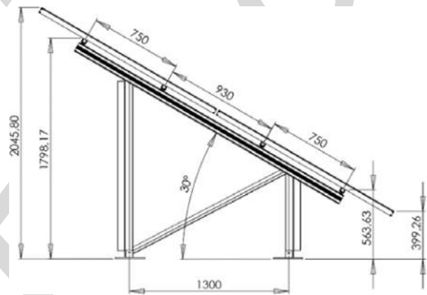
Fig. 10. Design dimensions (mm) of the PV structural base—side view.
