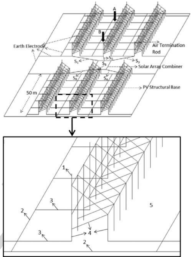
Fig. 9. Real-scale simulation model for a 150-kW solar park—with nonisolated L.P.S.
