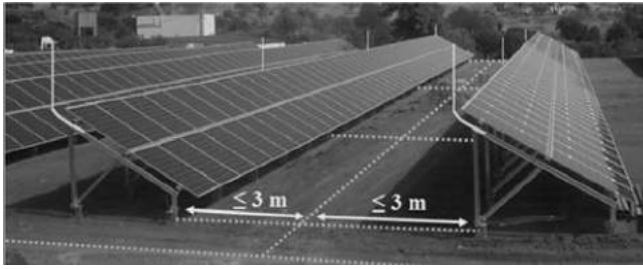
Fig. 7. Example of nonisolated L.P.S and earthing design for large-scale solar field applications.
