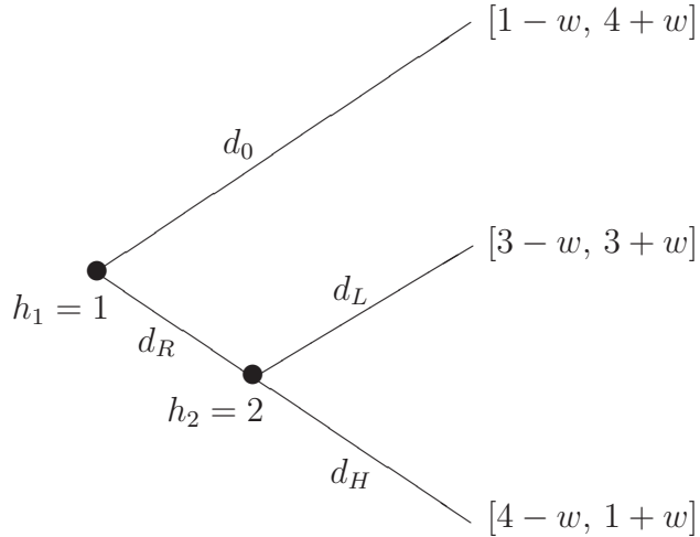
Figure 1: Multistage Decisions
