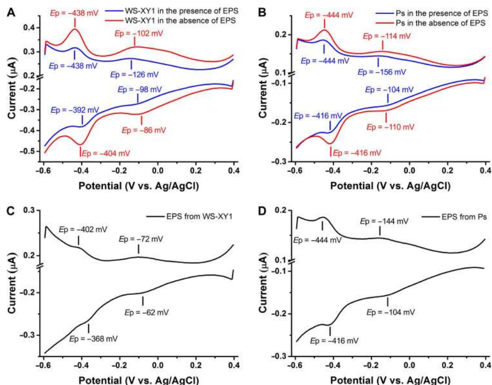
Fig. 6. DPV of cells and EPS of WS-XY1 and Ps . (A and B) DPV of WS-XY1 (A) and Ps (B) cells in the presence and absence of EPS. (C and D) DPV of EPS extract from WS-XY1 (C) and Ps (D) strains.
