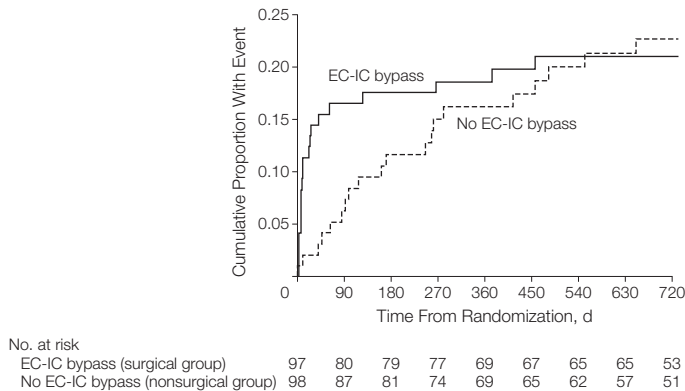
Figure 3. Kaplan-Meier Cumulative Curves for the Analysis of the Primary End Point
