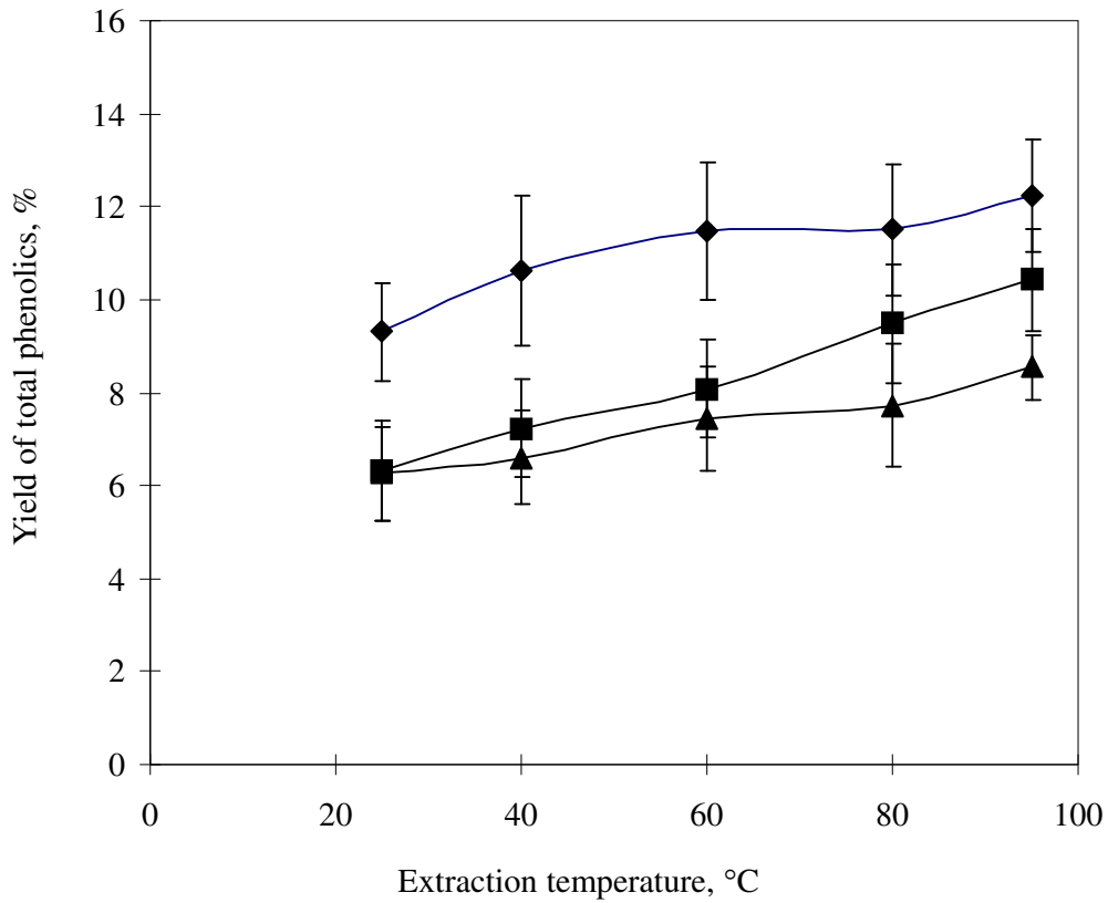
Fig. (4). The effect of extraction temperature on the yield of total phenolics for different solvent solid/ ratios. Extraction time was 2 min and the particle size of 40 mesh: \blacktriangle , 1:09; \blacksquare , 1:15; \blacklozenge , 1:25.
