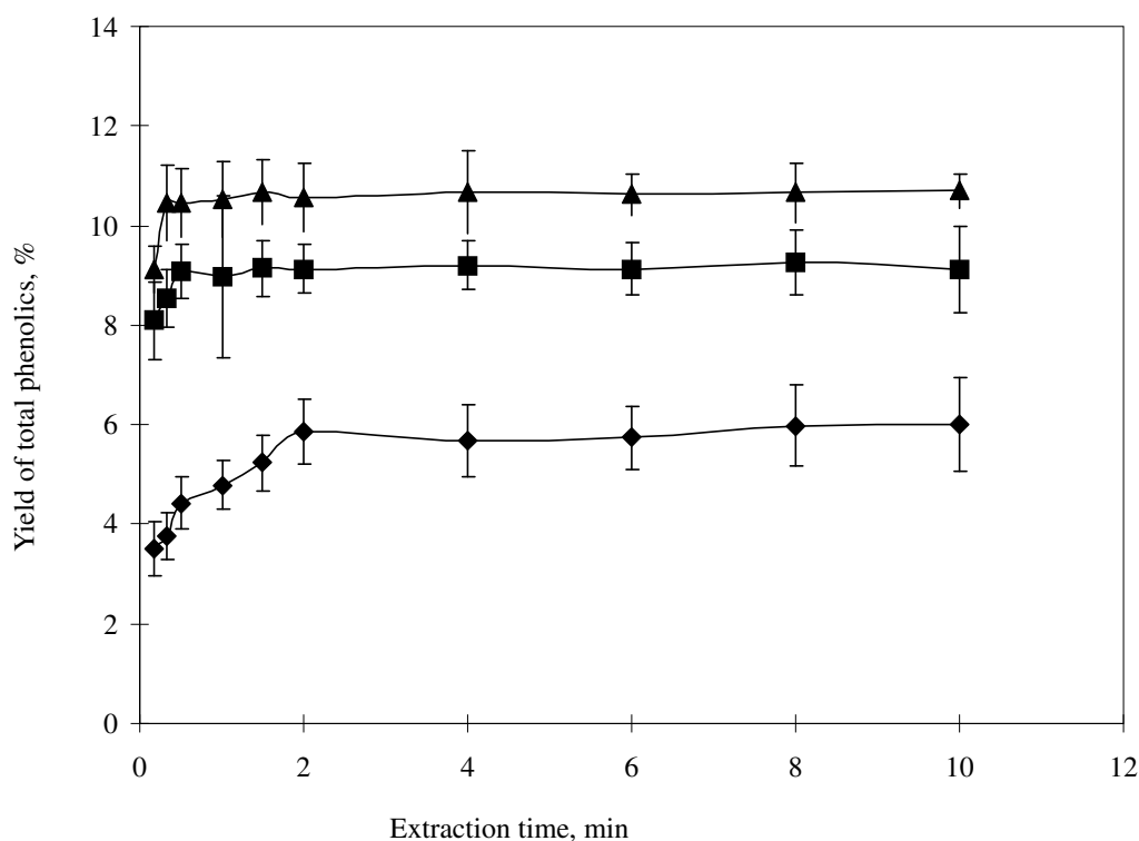
Fig. (3). The kinetics curves of water extracted total phenolics yield. The water extraction was done using a ratio of solvent to solid of 15: 1 and particle size of 40 mesh. \blacklozenge , 25°C; \blacksquare , 60°C; \blacktriangle , 95°C.
