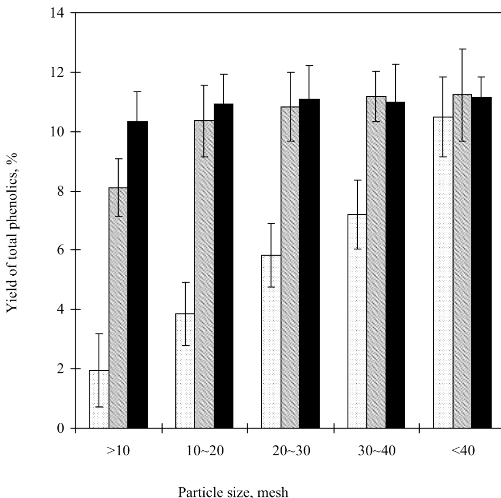
Fig. (6). The effect of particle size on the yield of total phenolics with different extraction times (2, 20 and 60 min). The extraction temperature was at 60°C. □, 2min; ▨, 20min; ■, 60min.
