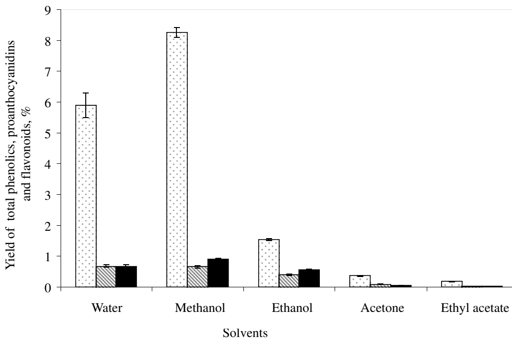
Fig. (1). The effect of different solvents on the yield of total phenolics, proanthocyanidins and flavonoids from the marc of pomegranate peels. Extraction was conducted at a temperature of 40 ^{\circ} C, a solvent/solid ratio of 15:1, a particle size of 40 mesh and an extraction time of 240 min: \square , Total phenolics; \square (hatched), Proanthocyanidins; \blacksquare , Flavonoids.
