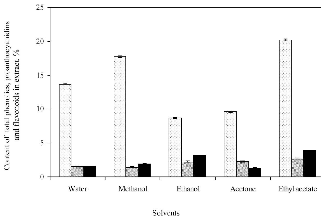
Fig. (2). The effect of different solvents on the content of total phenolics, proanthocyanidins and flavonoids from the marc of pomegranate peels (PMP) in the extract (g dried extract/100 g PMP). Extraction was conducted at a temperature of 40 °C, a solvent/solid ratio of 15:1, a particle size of 40 mesh and an extraction time of 240 min. □, Total phenolics; ▨, Proanthocyanidins; ■, Flavonoids.
