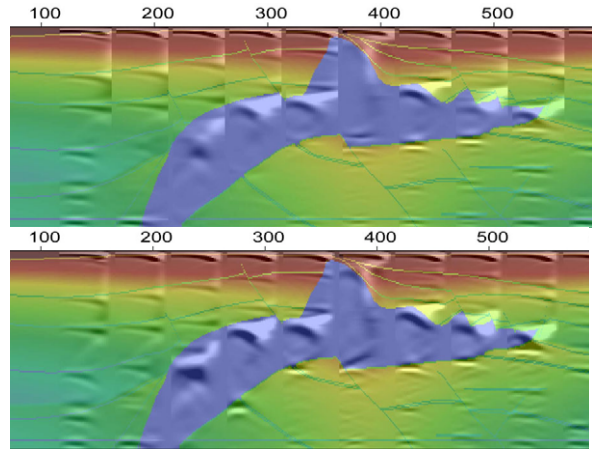
Figure 5. Angle domain image gathers for the SEG/EAGE Salt model.
