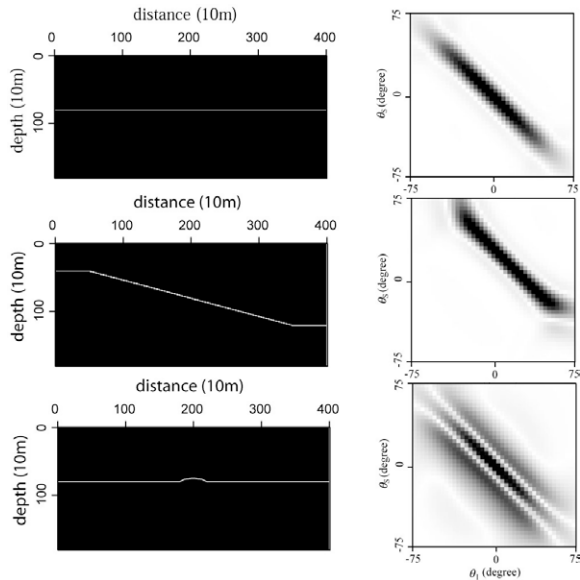
Figure 2. The local image matrices for typical structures. From upper to bottom are for flat, dipping and curved reflectors. On the left are velocity models and on the right are image matrices. For details see the text.
