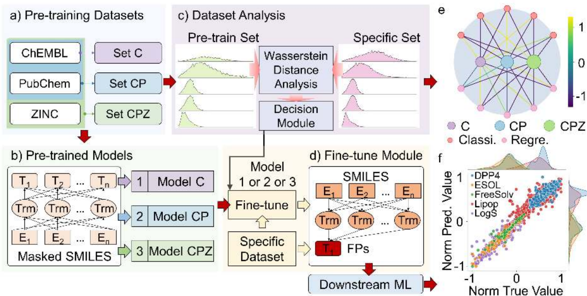
Figure 1: Illustration of the self-supervised learning platform. a Three public datasets are involved in the pre-training datasets module (blue rectangle). Set C only contains the ChEMBL dataset. Set CP consists of ChEMBL and PubChem datasets, and Set CPZ contains ChEMBL, PubChem, and ZINC datasets. b Based on those three datasets, three pre-trained models (green rectangle) are obtained by self-supervised learning, which is Model C, Model CP, and Model CPZ, respectively. c The dataset analysis module (purple rectangle) contains the Wasserstein distance analysis module and decision module. It will point to the best pre-trained model for a specific dataset. d The fine-tune module (yellow rectangle) fine-tunes the pre-trained model using a specific dataset. Finally, the fingerprints are generated from the fine-tuned model and used as input for the downstream machine learning tasks. e , The correlations between pre-training datasets and downstream datasets, including 5 classifications (Classif.) and 5 regressions (Regre.) datasets, and pre-trained datasets C, CP, and CPZ. f Normalized predicted results of the fingerprints from pre-trained model C for DPP4, ESOL, FreeSolv, Lipophilicity (Lipop), and LogS five regression datasets.
