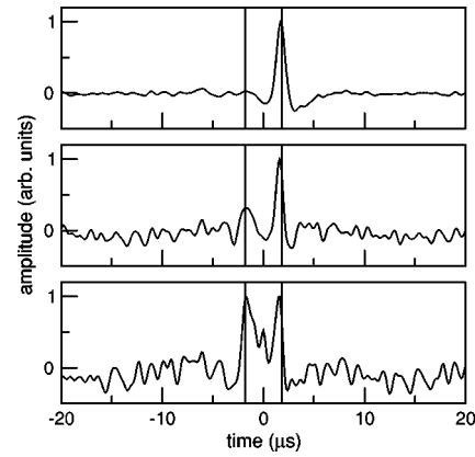
FIG. 2. Time correlation function in three different 30 \mu\text{s} windows of the recorded data. Data from the two detectors furthest from the source are used. The time used in the top panel (beginning at 5 \mu\text{s} , R/ct=0.40 ) is too early to see the acausal component, and the correlation is asymmetric. Between the times in the middle panel (beginning at 12.5 \mu\text{s} , R/ct=0.29 ) and the last panel (beginning at 25 \mu\text{s} , R/ct=0.20 ), the field becomes equipartitioned. The vertical lines indicate the expected arrival time of the surface wave, based on independent surface-wave velocity estimates.
