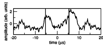
FIG. 5. Time correlation using only the sign bit of the data.
