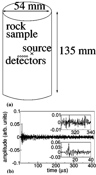
FIG. 1. (a) Experimental setup, 5 detectors starting 5 mm from the source with 5 mm spacing. (b) Typical data from the experiment. The lower inset shows the first arrivals and the upper inset shows a portion of the multiply scattered signal used in this experiment.
