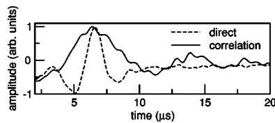
FIG. 4. Comparison of the retrieved Green function and the directly measured Green function; both are normalized to their peak amplitudes. They agree kinematically although high frequencies are suppressed in the retrieved Green function.
