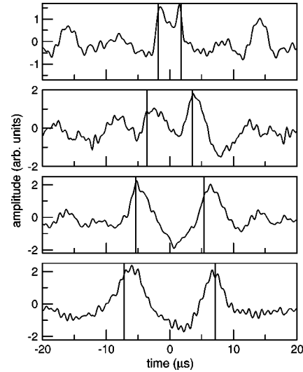
FIG. 3. Time correlation function for different offsets, each using 3 windows 30 \mu\text{s} in length. Top panel: Offset 5 mm, windows starting at 17.5 \mu\text{s} , R/ct=0.1 . Second panel: Offset 10 mm, windows starting at 30, 120, and 190 \mu\text{s} , R/ct=0.06 . Third panel: Offset 15 mm, windows starting at 80 \mu\text{s} with R/ct=0.13 . Bottom panel: Offset 20 mm, windows starting at 157.5 \mu\text{s} , with R/ct=0.03 . To ensure that each window represents an independent member of the ensemble, a 5 \mu\text{s} gap is left between consecutive windows.
