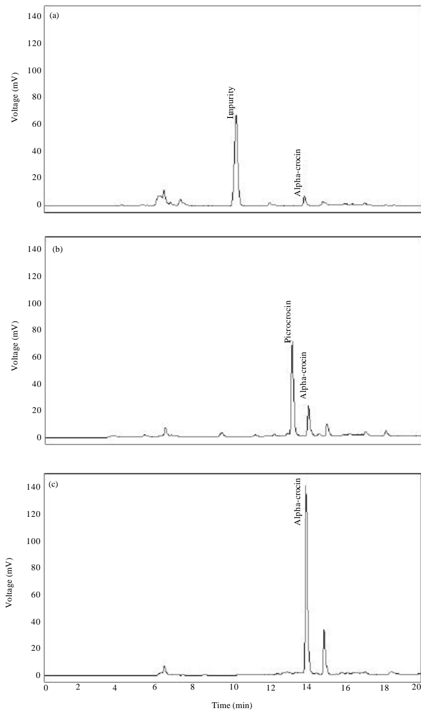
Fig. 3: Chromatograms of samples ( 50 \mu\text{g mL}^{-1} ) at 250 nm, (a) Fluka crocin, (b) saffron stigma extract samples and (c) crystallized crocin. A gradient method was used which mobile phase composition was changed from 20 to 80% MeCN in water at 20 min
