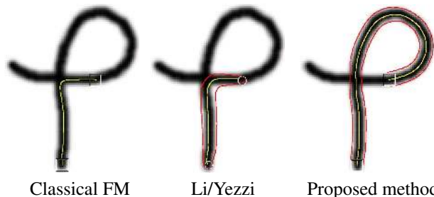
Figure 8. Comparison of the different methods when encountering a crossing. Only the proposed method goes from the start to the ending point following the natural path for vessel extraction.
