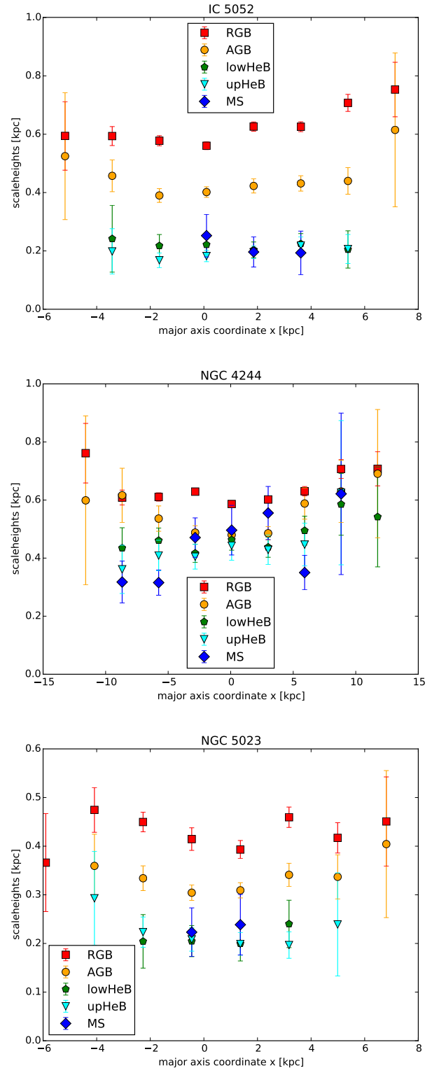
Fig. 5. Disk scale heights at different radial position in the three low-mass edge-on galaxies IC 5052, NGC 4244, and NGC 5023 ( top to bottom ). Colors are the same as in Fig. 3.
