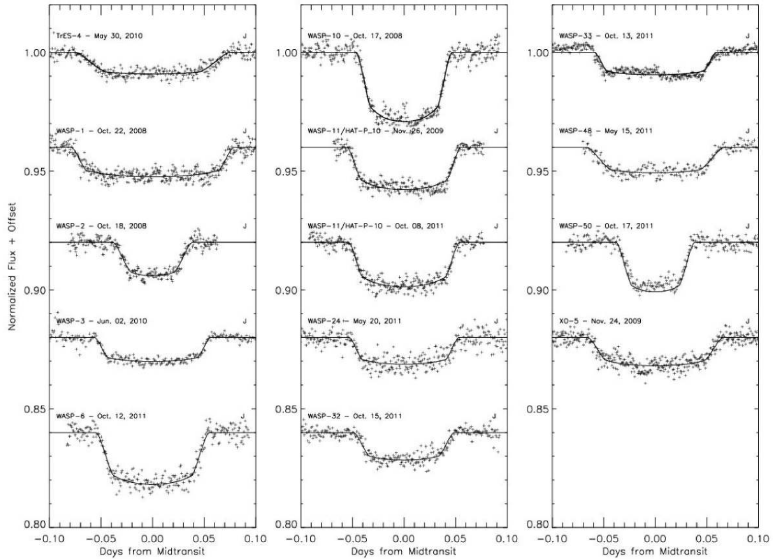
Figure 1b: Exoplanet Transits observed in the near-IR with the KPNO 2.1m telescope
