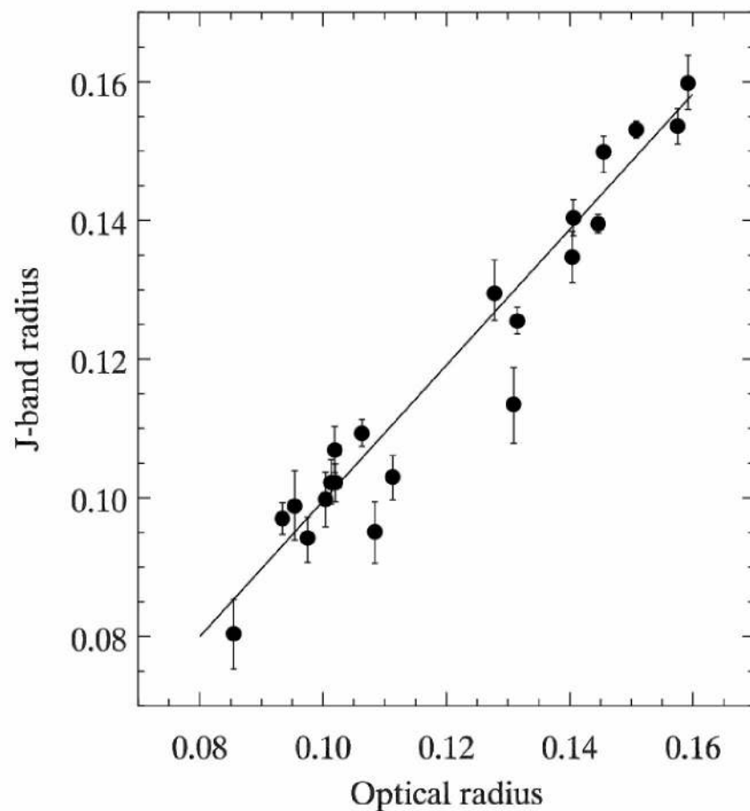
Figure 3: Ratio of planetary to stellar radius, R_p/R_* , from MCMC fitting to our J-band transit curves (ordinate, from Table 3), compared to published optical radii for the same planets. We exclude HAT-P-27/WASP-40 due to its much larger error. The solid line is a least squares fit (see text), and it differs negligibly from the null hypothesis that the derived planetary radii are independent of wavelength (see text).
