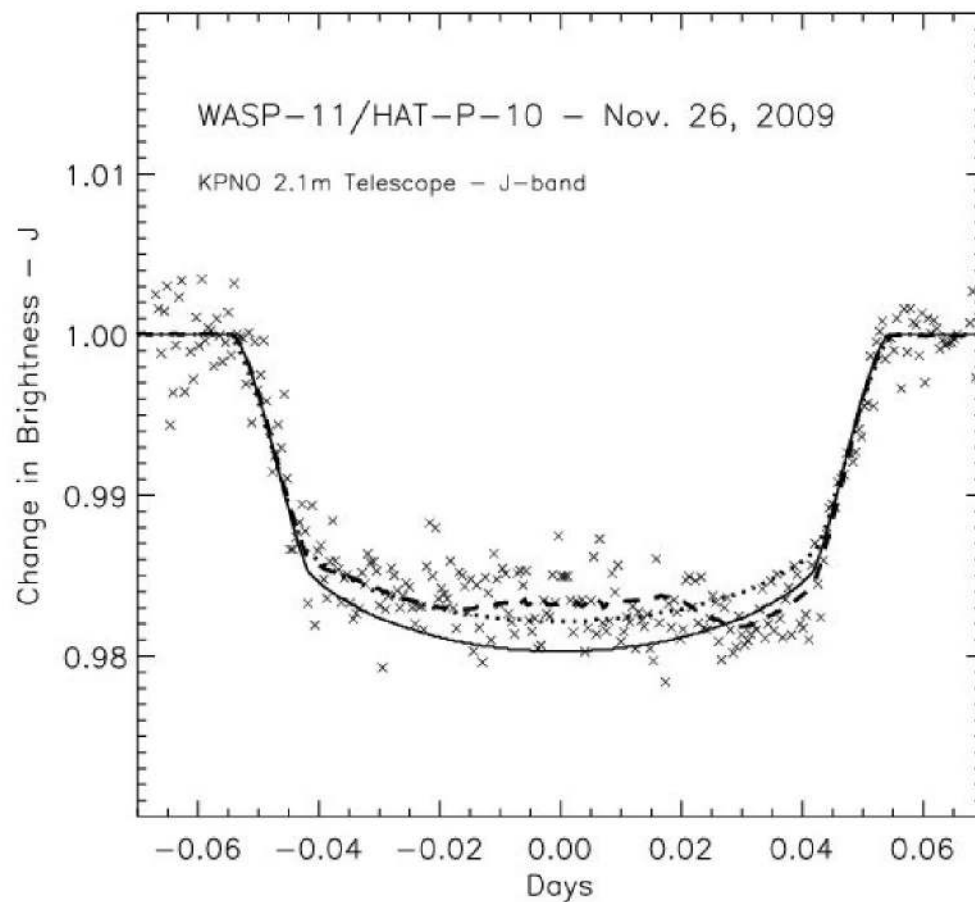
Figure 4: Observed transit of HAT-P-10/WASP-11 on 2009 November 26 at the KPNO 2.1m telescope through a J-Band filter. The solid line is the model derived from the literature parameters. The dotted line is our fit to the entire depth of the transit. The dashed line is the literature model but with part of the stellar surface covered by starspots with temperature \sim 6\% lower than the effective temperature of the star (4920 K).
