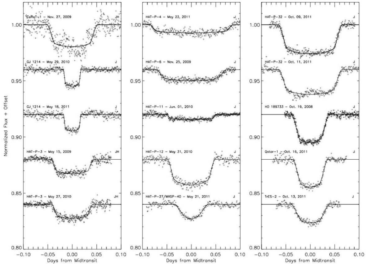
Figure 1a: Exoplanet Transits observed in the near-IR with the KPNO 2.1m telescope
