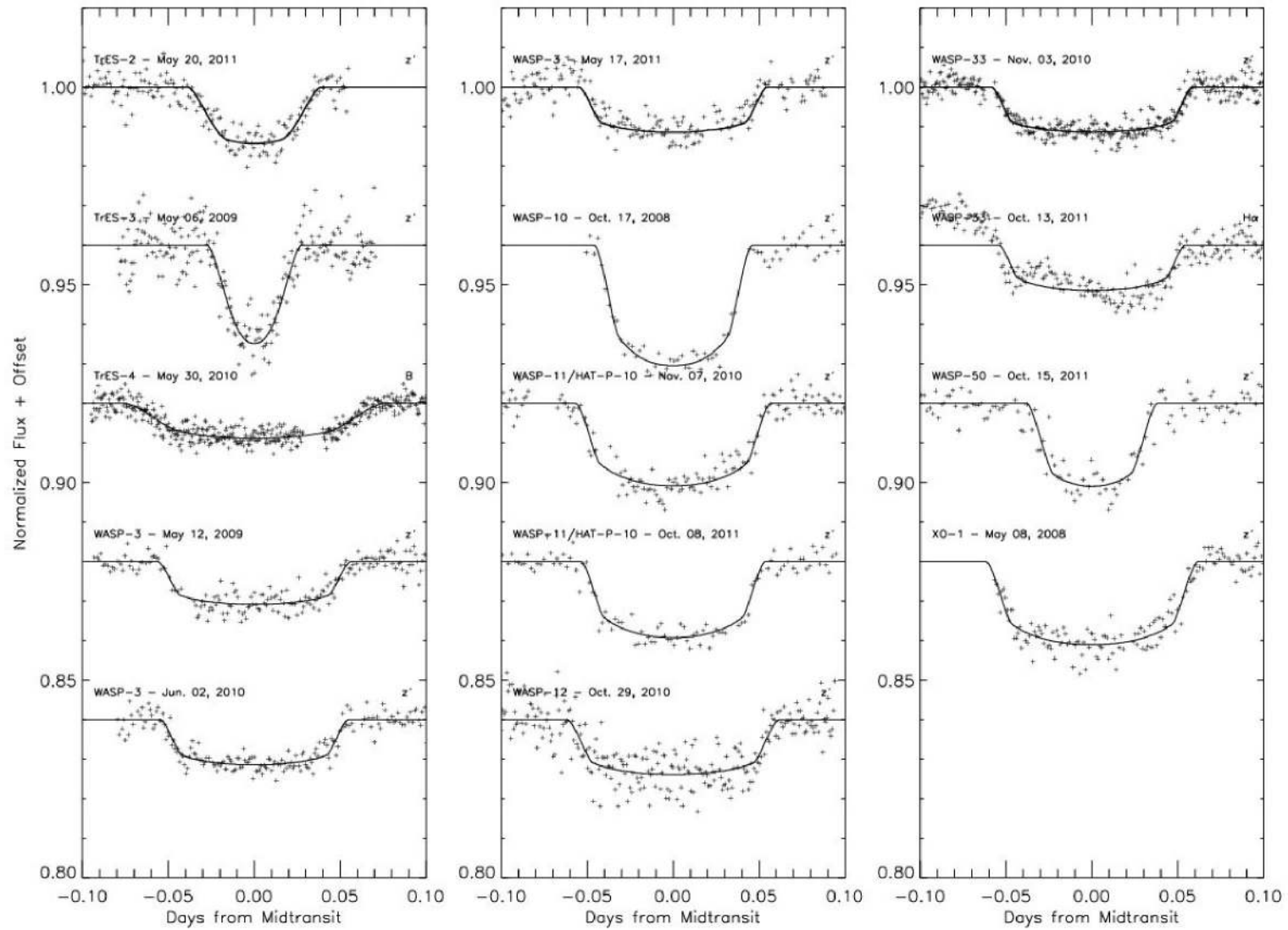
Figure 2b: Exoplanet Transits observed in the visible with the KPNO Visitor Center 0.5m telescope.
