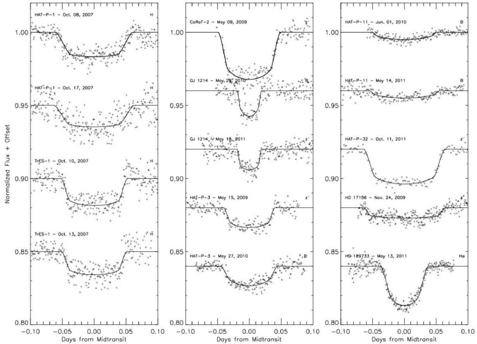
Figure 2a: Exoplanet Transits observed in the near-IR with the KPNO National Solar Observatory McMath-Pierce 2.0m telescope (left column) and in the visible with the KPNO Visitor Center 0.5m telescope.
