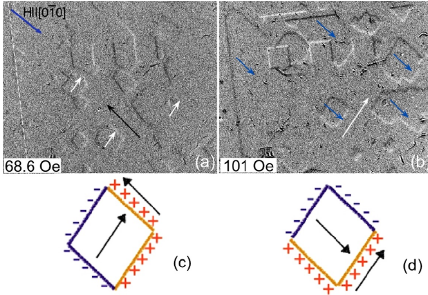
Fig.2. (a-b) Magneto-optical images of two-stage axial remagnetization at T=5\text{K} . Images of the same area as in Fig.1 are referenced to the initial monodomain \mathbf{M}_1 -state with \mathbf{M}_1 \parallel \text{EA}_2 (black arrow) formed after application of \mathbf{H} \parallel [010] . Subsequent application of \mathbf{H} \parallel [1-10] promotes nucleation and growth of domains with \mathbf{M}_2 \parallel \text{EA}_1 (white arrows) (a). These domains have bright and dark boundaries associated with magnetic charges sketched in (c). In this first remagnetization stage, the \mathbf{M}_2 domains have 90^\circ - 2\alpha DWs. At larger H , the \mathbf{M}_2 domains expand and form a monodomain state (not shown) where then new domains with \mathbf{M}_3 \parallel -\text{EA}_2 (blue arrows) appear and grow (b). These domains have bright and dark bottom and top-side boundaries associated with the magnetic charges sketched in (d). In the second rotation stage, the \mathbf{M}_3 domains have 90^\circ + 2\alpha DWs. For both stages the DWs are oriented along EA1 and EA2.
