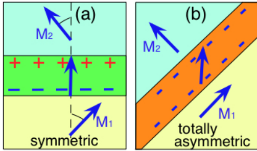
Fig.3 Sketch of symmetric and asymmetric 90^\circ Neel domain walls. In the symmetric case (a), magnetic charges \rho_m changes sign across the DW, whereas they have one sign in the asymmetric Neel wall (b). Details of the \rho_m distribution are presented in the Supplemental information [23]. The range of stray fields H_s for (b) is much larger, similar to H_s of a charged line decaying with distance as 1/R , compared to a dipole of +/- lines with H_s \sim 1/R^2 in (a). Blue arrows show magnetization vectors in the domains and inside the Neel DW.
