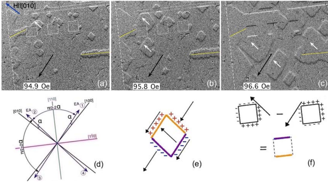
Fig.1 Magneto-optical images of the nucleation and growth of domains during perpendicular remagnetization at T=5\text{K} (a-c). The orientation of the easy axes EA1 and EA2 and the crystal axes is shown in (d). The sample has 3 etched 150 \times 150 \mu\text{m} square apertures and a slit with sides parallel to [110] and [1-10] (white lines). The yellow lines indicate scratches in the sample. The sample is initially polarized into a monodomain state (not shown) with \mathbf{M}_1 \parallel -\text{EA1} (black arrow) by application of \mathbf{H}=1\text{kOe} \parallel [-100] and switching off H . Panels (a-c) present subsequent images in \mathbf{H} \parallel [010] after subtraction of the initial polarized \mathbf{M}_1 -state picture to enhance the contrast of new domains. Rhombus-shaped domains with \mathbf{M}_2 \parallel \text{EA2} (white arrows) appear and grow with increasing H . They have bright and dark 90^\circ + 2\alpha domain walls (DWs) oriented along EA1 and EA2. Domains nucleating at the scratches have zigzag boundaries. The DW bright and dark contrast reveals Up and Down directed stray fields due to + and - magnetic charges at the DWs (e). Visualization of the stray fields at the edges of the apertures allows monitoring of the \mathbf{M} components in adjoining areas. In the subtracted image (c), the square aperture and the slit sides where the magnetic charge inverts sign, become visible upon the expansion of \mathbf{M}_2 domains as sketched in (f). Our MOI resolution is \sim 2\mu\text{m} , but the stray fields diverge in a range wider than 2\mu\text{m} .
