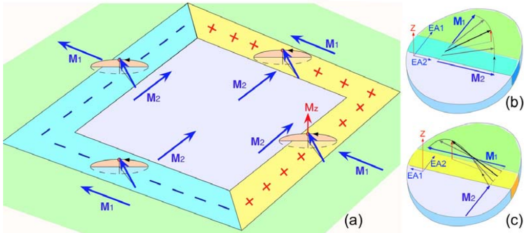
Fig.4 Sketch of asymmetric Neel domain walls modified by Dzyaloshinskii-Moriya interactions. \mathbf{M}_1 \parallel \text{EA}_1 in the initial state and \mathbf{M}_2 \parallel \text{EA}_2 in the nucleating domain are both in the film plane. Due to the DMI, magnetization in the Neel DW tilts slightly out of the plane, as shown by ellipses with their small axis along the film normal Z . Within the DWs, \mathbf{M}
