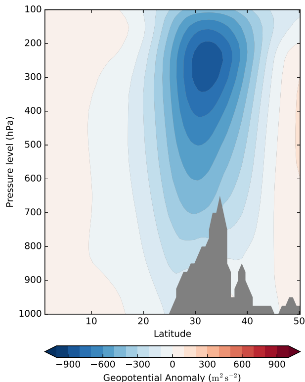
FIG. 6. Vertical structure of geopotential anomaly for the hundred strongest winter EPEs. Construction as in Fig. 4(b), with the cross-section taken along the line given in that figure ( 68^{\circ}\text{E} ). Grey areas indicate the presence of orography.
