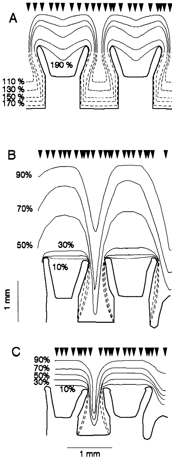
Figure 2. Contour maps of the oxygen boundary layers surrounding Stylophora pistillata coral polyps. Each map was constructed from measurements of oxygen profiles taken from 10 different colonies. Further details are as in the legend to Figure 1 (symmetry duplication was not used).
