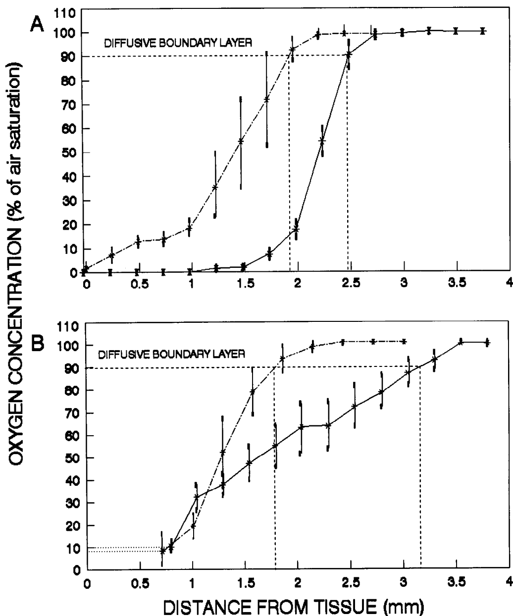
Figure 3. Oxygen concentrations perpendicular to the oral disk opening of the corals Favia fava (A) and Stylophora pistillata (B) in calm water (continuous lines) and with a 5-cm/s current (dashed lines). Means \pm SD; n: A-calm = 4, A-current = 3, B-calm = 5, B-current = 7.
