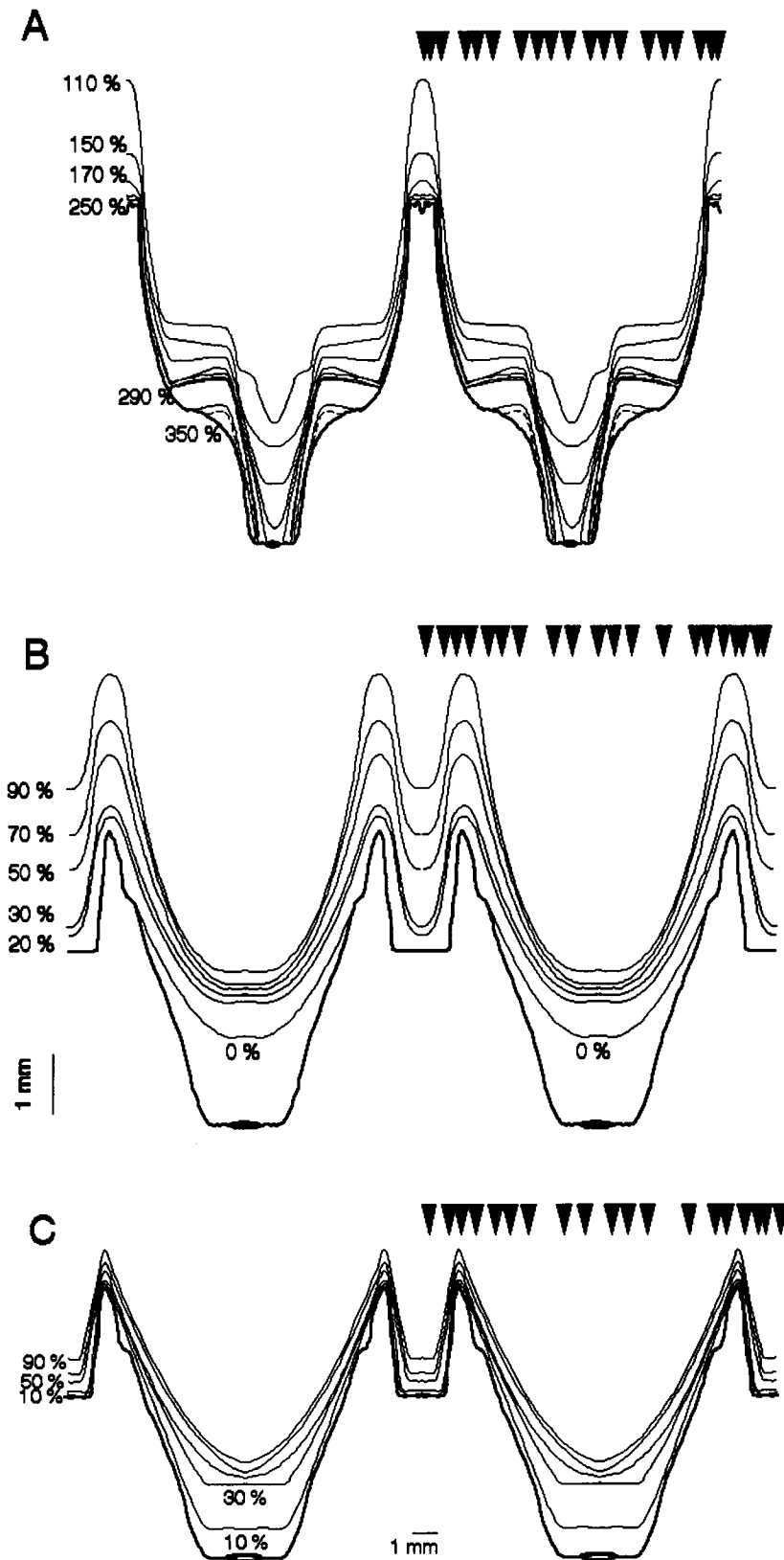
Figure 1. Contour maps of the oxygen boundary layers surrounding Favia fava coral polyps. Each map was constructed from measurements of oxygen profiles taken from 10 different colonies. Arrows indicate points of profile measurements. Tissue surface is marked in bold lines. Dashed lines mark estimated values where continuous measurements were not possible. For better illustration, maps were duplicated by left symmetry. (A) Oxygen boundary layer under light conditions of 980 \mu\text{E} \cdot \text{m}^{-2} \cdot \text{s}^{-1} . (B) Oxygen boundary layer in darkness. (C) Oxygen boundary layer under a 5-cm/s current, in darkness.
