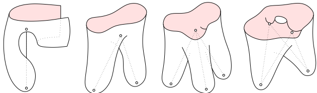
Figure 1: From left to right: a one-, two-, three-, and four-legged local maximum of the elevation function. In the examples shown, the outer normals at the endpoints of the legs are all parallel (the same). Each of the four types also exists with anti-parallel outer normals in various combinations.
