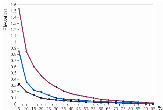
Figure 9: The percentage of maxima with elevation exceeding the threshold marked on the vertical axis. From top to bottom: the curves for the three-legged, four-legged, and two-legged maxima.
