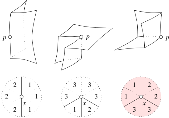
Figure 8: The three sheets of \mathbb{Q} after cutting and gluing the neighborhood of a triple point p in \mathbb{P} , at the top, and the corresponding pairing patterns in the neighborhood of x , at the bottom. The (shaded) Mercedes star is necessary for a three-legged maximum.
