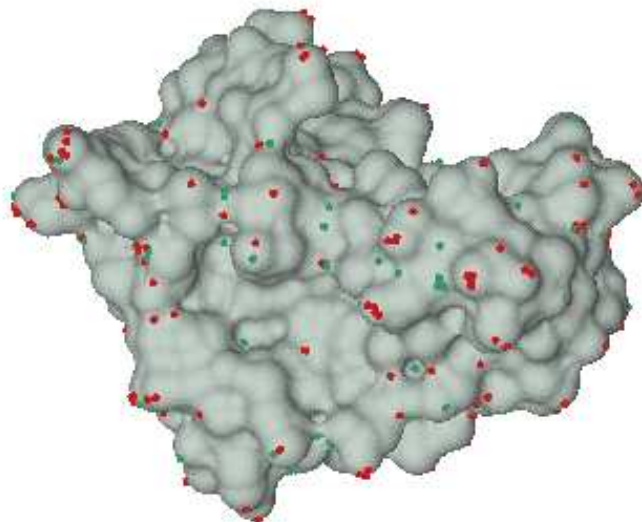
Figure 10: The one hundred pairs of maxima with highest elevation. The heads are marked by light and the feet by dark dots.
