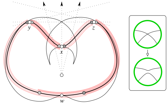
Figure 6: The four white points share the same normal direction, as do the four light shaded and the four dark shaded points. The strips indicate the pairing, which switches when the height function passes through the vertical direction. The insert on the right illustrates the effect of surgery at y and z on the pedal curve.
