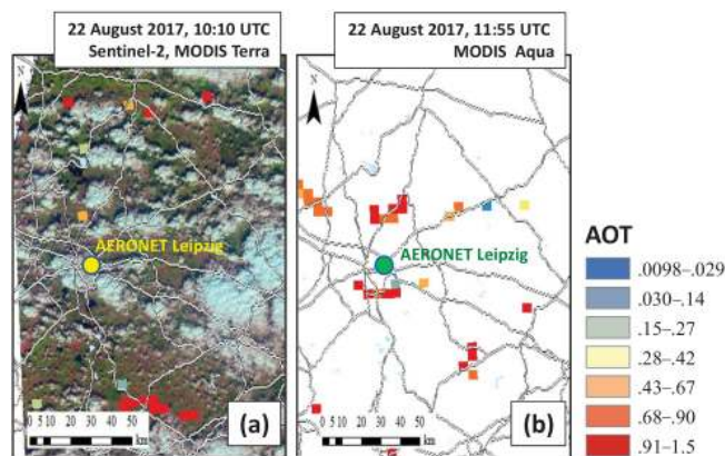
Figure 8. (a) Sentinel-2 cumulus cloud fields (bluish-white) and integrated MODIS Terra color-scaled 550 nm AOT values for 3 \text{ km} \times 3 \text{ km} cloud-free areas (Leipzig, overpass at 10:10 UTC), and (b) respective MODIS Aqua 550 nm AOT retrievals (Leipzig, overpass at 11:55 UTC). The yellow (a) and green (b) circles indicate the AERONET Leipzig site. Many red squares (AOT of 0.9–1.5) were retrieved from the MODIS observations north and south of the AERONET station.
