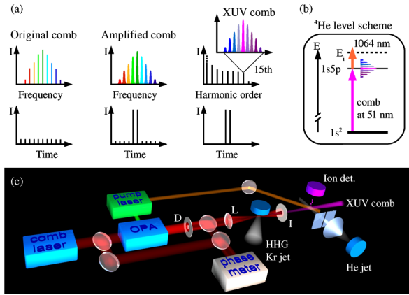
FIG. 1 (color online). (a) Spectral and temporal structure of the generated light (left to right): FC of the continuous coherent pulse train from the FC laser, the cosine-modulated spectrum of a pair of amplified pulses, and odd harmonics of the amplified FC laser pulses each containing a cosine-modulated XUV comb corresponding to the XUV pulse pair. (b) Simplified ^4\text{He} level scheme, XUV comb excitation at 51.5 nm from the 1s^2 ground state to the 1s5p excited state and state-selective ionization by a pulse at 1064 nm. (c) Schematic of the experimental setup. D : beam mask, L : focusing lens, f = 50 cm, I : iris to separate XUV from IR. The pump laser provides both the 532 nm for pumping the OPA as well as 1064 nm for ionization of helium.
