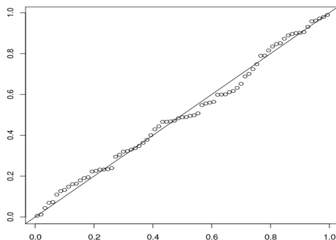
FIGURE 7. Example of PP-plot for the original sample.
