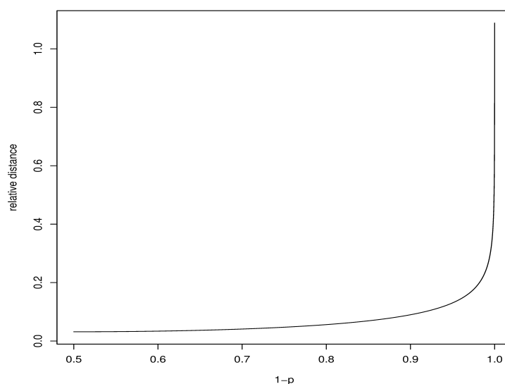
FIGURE 1. Relative distance between quantiles of order p computed with \mathcal{N}(0,1) and Student(4) models.
