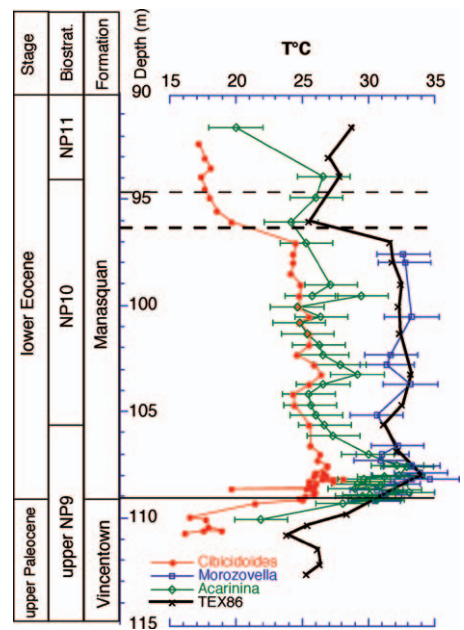
Figure 4. Sea surface temperatures as computed from (1) planktonic foraminifera δ 18 O and (2) the TEX 86 . The oxygen isotope-based curves were derived assuming seawater δ 18 O sw of −0.5‰ (SMOW) using standard paleotemperature equation (Erez and Luz, 1983). The errors bars on the planktonic foraminifera curves reflect the range of estimated temperatures associated with just a ±0.5‰ uncertainty in δ 18 O sw .
