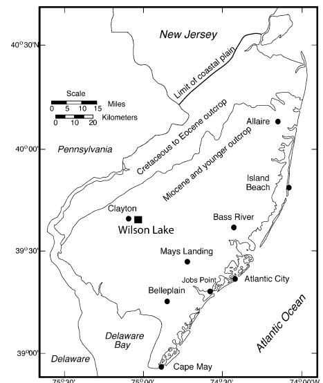
Figure 1. Location map showing the location of Wilson Lake (~39°39'N, 75°2'W) and other USGS and ODP cores (modified from Miller, 1997).
