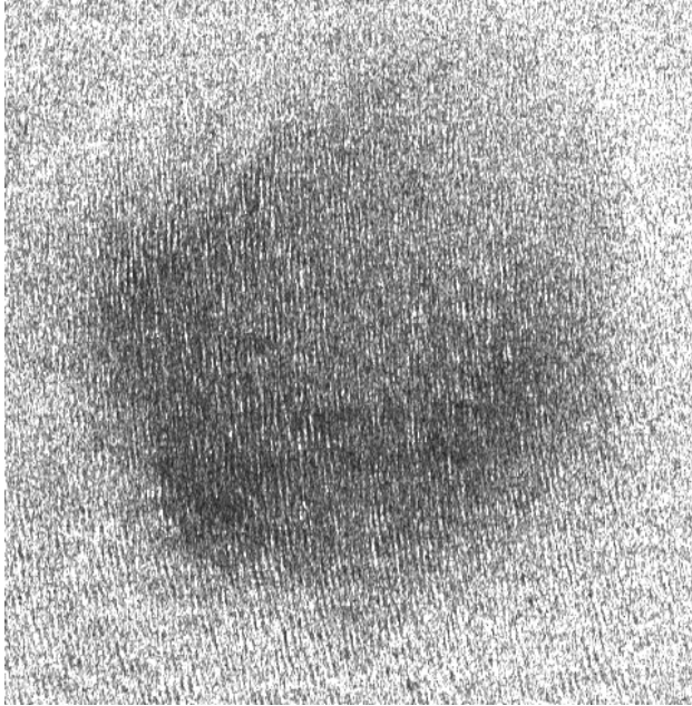
Figure 2. A 10 \times 10 \text{ km} subsene from Figure 1, zoom onto the eye of hurricane Ivan, taken on September 10.
