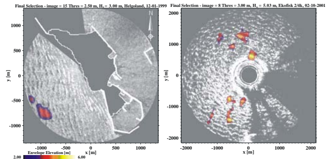
Figure 10. Dominant wave groups from Heligoland (left) and from Ekofisk (right). Transparently overlaid are the wave envelopes of the dominant wave groups with a chosen minimum area size.
