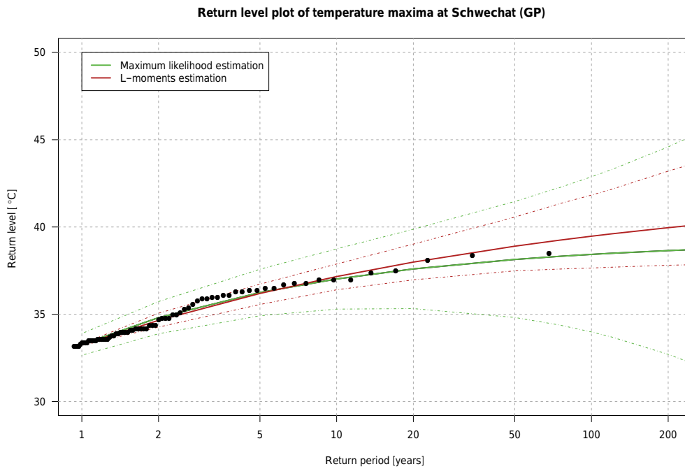
Figure 3. Return level plot of temperature maxima at Schwechat. Return level estimation is based on the threshold excess approach with two different parameter estimation methods (MLE and LMOM estimation). Solid lines show the mean estimate, while dashed lines indicate the 95 % confidence intervals for the fitted functions.
