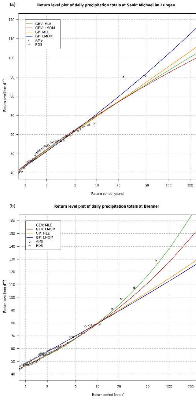
Figure 6. Return level plots of daily rainfall events at the hot spot in (a) Sankt Michael im Lungau, which is located in the Central Eastern Alps, and (b) Brenner pass, located at the Austro-Italian border. Return level estimation is based on the block maxima approach and on the threshold excess approach with two different parameter estimation methods (MLE and LMOM estimation). Based on the CRMSE 10 , GP fitted on the basis of LMOM estimation was found to be the most appropriate method for Sankt Michael, while GEV with MLE was found to be most suitable at Brenner. Please note that functions are plotted without associated confidence intervals for the sake of clarity.
