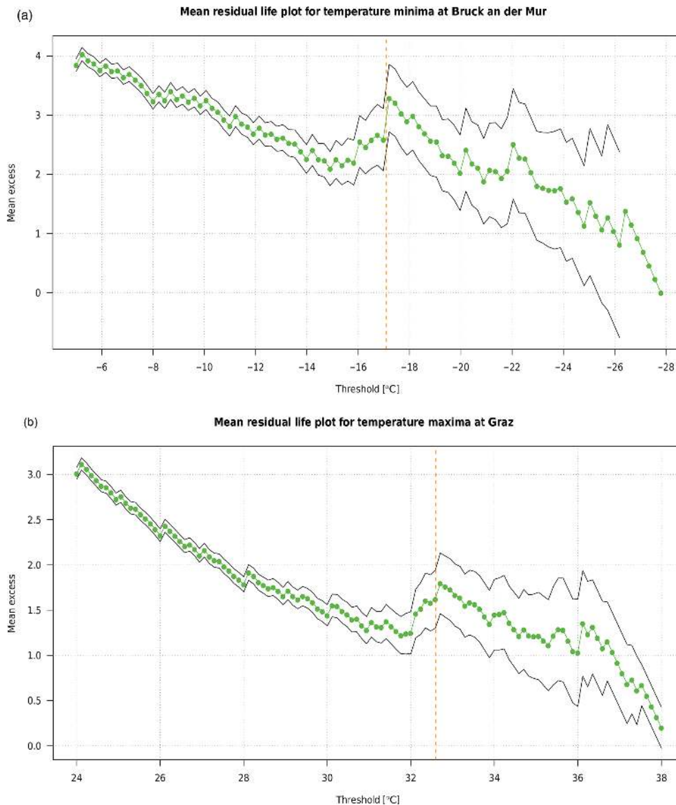
Figure 8. Mean residual life plots of (a) temperature minima the hot spot in Bruck an der Mur and (b) temperature maxima at Graz. Black lines indicate the 95 % confidence interval for the mean excess and orange lines indicate the threshold selected by means of the square-root rule.
