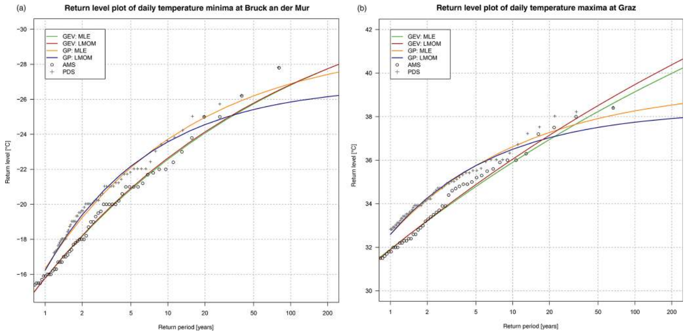
Figure 7. Return level plots of (a) temperature minima at Bruck an der Mur and (b) temperature maxima at Graz. Return level estimation is based on the block maxima approach and on the threshold excess approach with two different parameter estimation methods (MLE and LMOM estimation). Based on the CRMSE_{10} , GP fitted on the basis of MLE was found to be the most appropriate method for both Bruck an der Mur and Graz.
