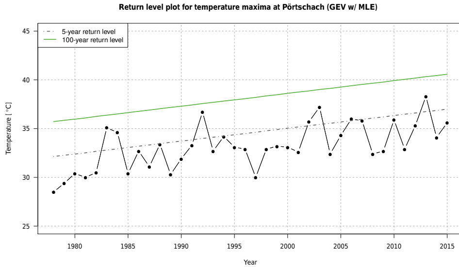
Figure 2. Return level plot of temperature maxima at Pörschach (Carinthia) with linear trend correction. The trend is visible in the lines depicting the 5-year return level (gray dashed line) and the 100-year return level (green solid line). This is an illustrative example of temperature trends that are commonly observed at the selected stations for both temperature maxima (increasing trend) and temperature minima (decreasing trend).
