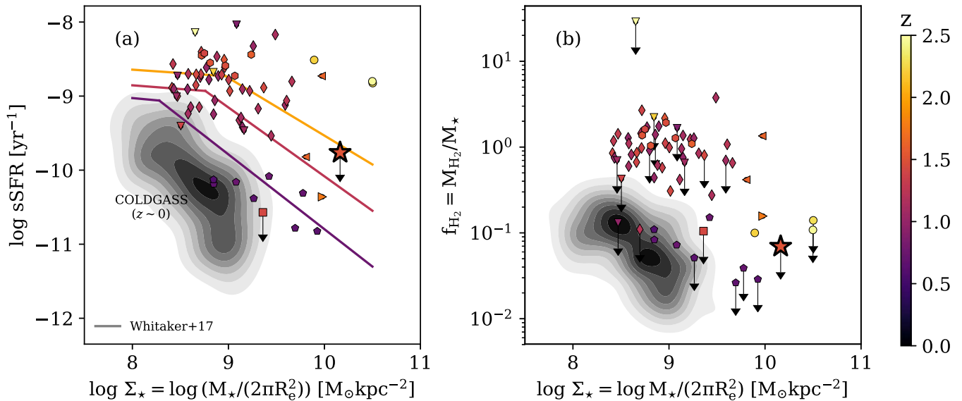
Figure 5. Specific star formation rate and \text{H}_2 gas fraction vs. stellar mass surface density for galaxies at z \sim 0 (gray contours, COLDGASS survey) and at higher redshift (symbols, colored by redshift). Local galaxies lie offset in sSFR (left) and f_{\text{H}_2} (right) at fixed stellar density, as expected. Broken power law relations between sSFR and \Sigma_* for all galaxies at (z) = 0.75, 1.25, and 1.75 from Whitaker et al. (2017) are indicated by solid lines in panel (a). Although some galaxies at fixed density and redshift overlap in sSFR (a), gas fractions at all redshifts drop dramatically for the most dense galaxies ( \Sigma_* \gtrsim 5 \times 10^9 M_\odot \text{kpc}^{-2} , b).
