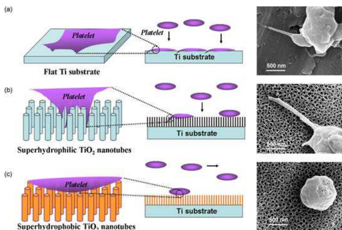
Fig. 14. Schematic illustration of the quantity and morphology of platelet and corresponding interactions on the three kinds of surfaces. (a) Plain Ti substrate; (b) Superhydrophilic TiO 2 nanotubes; and (c) Superhydrophobic TiO 2 nanotubes.
