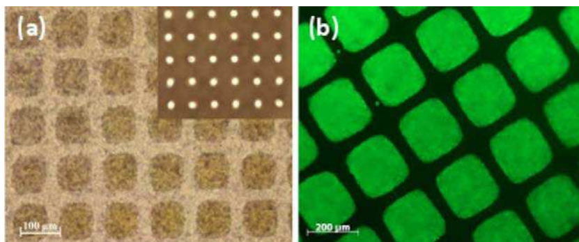
Fig. 5. (a) Optical micrograph of the as-obtained superhydrophilic-superhydrophobic pattern by focusing on the water droplet within the superhydrophilic regions. (b) Fluorescence microscopy image of the fluorescein probes on the as-prepared superhydrophilic-superhydrophobic micropattern.
