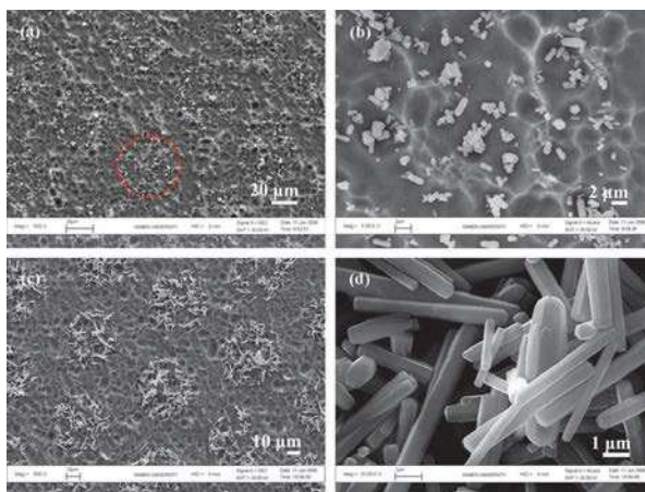
Fig. 9. SEM images of the patterned ZnO nanostructured micropatterns by liquid phase deposition at 90°C for different times: (a, b) 30 min; (c, d) 90 min.
