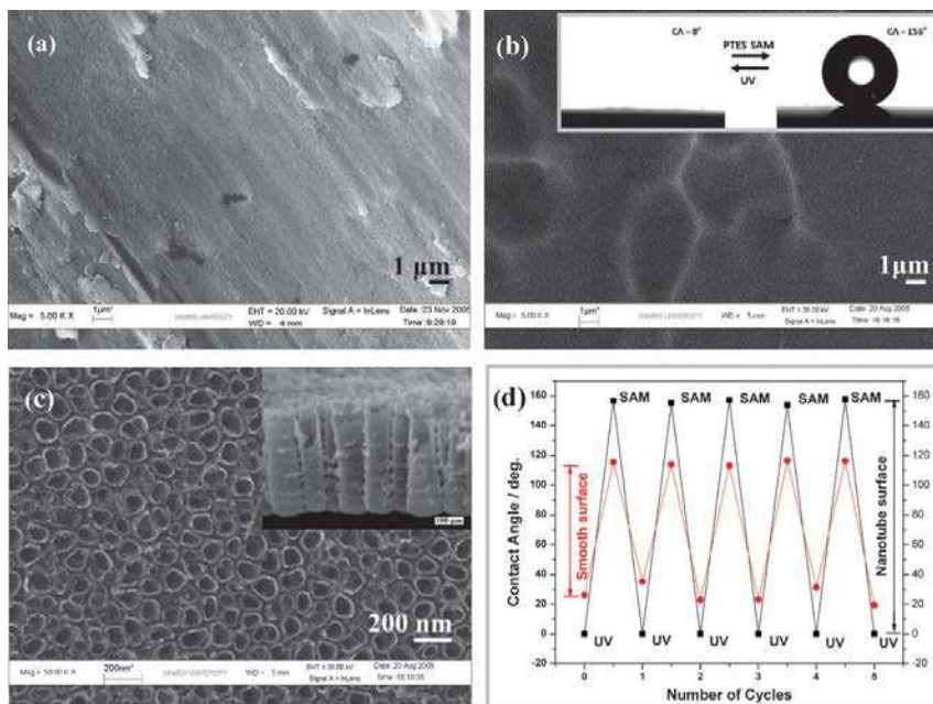
Fig. 1. SEM images of the mechanically polished and cleaned titanium substrate (a), low magnification of a nanotube structured TiO 2 film (b), and a higher magnification of the TiO 2 nanotube array film (c). Reversible surface wettability on a “flat” TiO 2 film and rough nanotube TiO 2 film by alternating SAM and UV photocatalysis (d). The inset of (b) shows the shape of a water drop on the PTES-modified and UV-irradiated TiO 2 nanotube array film. The inset of (c) shows the side view of a TiO 2 nanotube array film.
