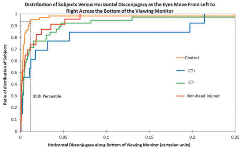
FIG. 1. Relative distribution of trauma patients and noninjured controls (y-axis) versus disconjucy (x-axis) to demonstrate that control subjects have the greatest proportion of patients with low horizontal disconjucy and positive CT patients have the highest proportion of patients with high horizontal disconjucy as the eyes move along the bottom segment of the box trajectory. Negative CT patients have a disconjucy in between positive CT and non-head-injured control subjects. Kruskal-Wallis' statistical analysis yielded a value of p < 0.05 for CT^+ and CT^- relative to noninjured controls. CT, computed tomography. Color image available online at www.liebertpub.com/neu
