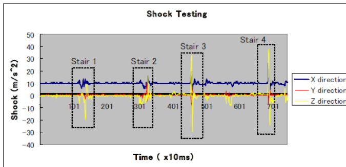
Figure 12. Shock Influence
