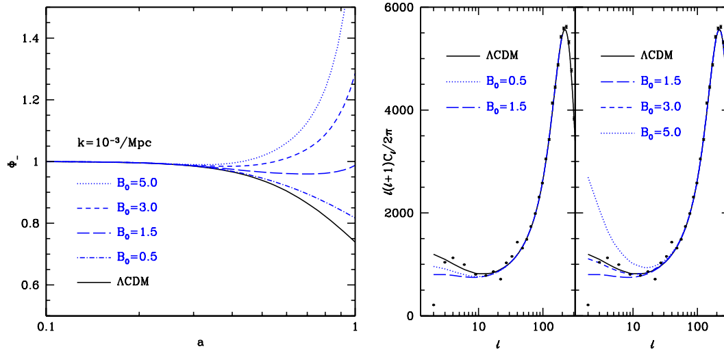
Figure 7: (Left) Evolution of the effective gravitational potential \Phi_{\text{eff}} (denoted as \Phi_- in the figure) versus the scale factor a (with the present value a = 1 ) on the scale k^{-1} = 10^3 Mpc for the \Lambda CDM model and f(R) models with B_0 = 0.5, 1.5, 3.0, 5.0 . As the parameter B_0 increases, the decay of \Phi_{\text{eff}} decreases and then turns into growth for B_0 \gtrsim 1.5 . (Right) The CMB power spectrum \ell(\ell+1)C_\ell/(2\pi) for the \Lambda CDM model and f(R) models with B_0 = 0.5, 1.5, 3.0, 5.0 . As B_0 increases, the ISW contributions to low multipoles decrease, reach the minimum around B_0 = 1.5 , and then increase. The black points correspond to the WMAP 3-year data [561]. From [545].
