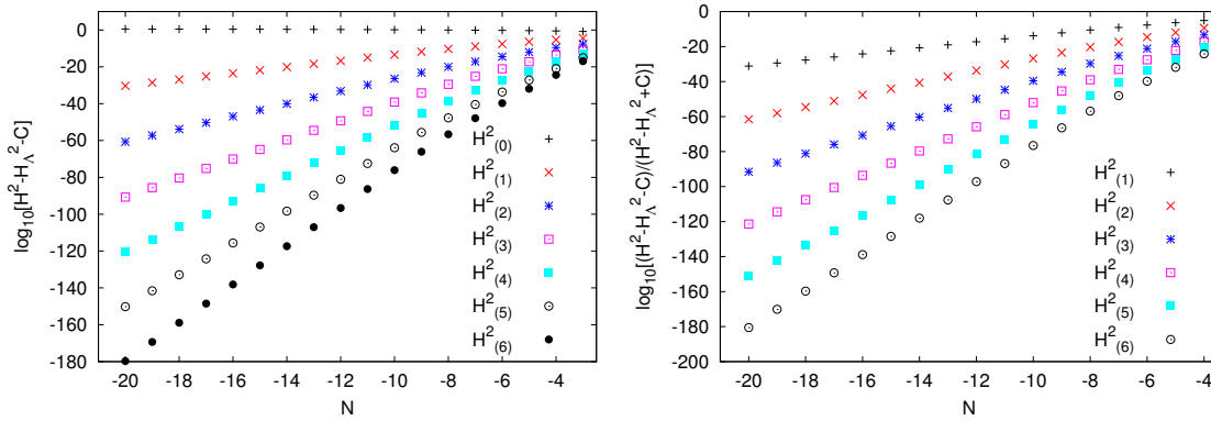
Figure 13: Plot of the absolute errors \log_{10}(|H^2 - H_\Lambda^2 - C_i|) (left) and \log_{10} \left[ \frac{|H^2 - H_\Lambda^2 - C_i|}{|H^2 - H_\Lambda^2 + C_i|} \right] (right) versus N = \ln a for the model (12.16) with i = 0, 1, \dots, 6 . The model parameters are \alpha = 10 and \lambda = 0.075 . The iterative method provides the solutions with high accuracy in the regime N \lesssim -4 . From [188].
