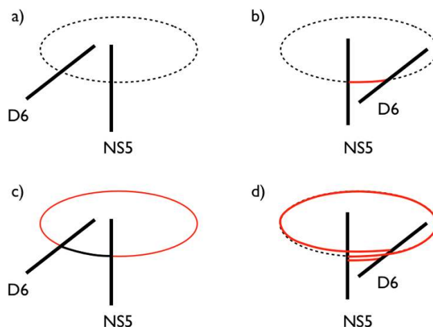
Figure 1. a) The T-dual of a D7-brane on a Taub-NUT is a D6- and an NS5-branes at points in the T-dual circle. b) As the D6-brane crosses the NS5-brane, an stretched D4-brane is created. c) Moving to larger values of \phi the D6-brane returns close to the NS5-brane. d) Creation of additional D4-branes in each crossing implies the monodromy in \phi . The additional brane creation in each crossing makes this construction differ from figure 1 in [17].
