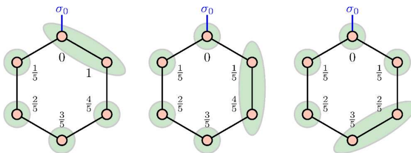
Figure 2. The U(1) charge of a \underline{5} hypermultiplet localized at a codimension-two fiber where the I_5 discriminant (green) degenerates to I_6 (red). Pick the red node where the section generating the Mordell-Weil group intersects the fiber. The number next to the node is the ratio of the U(1) charge relative to a \underline{1} hypermultiplet.
