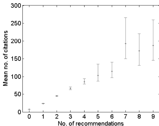
Figure 11. Relation between the number of recommendations of a publication and the average number of citations. The error bars indicate 95% confidence intervals.
