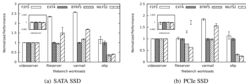
Figure 4: Performance results on the server system.
