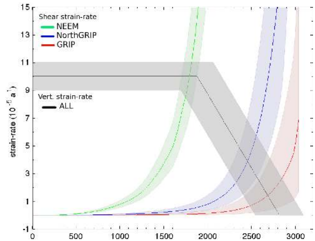
Figure 6. Evolution of the shear strain rates, D_{xz} , along the GRIP (red), NGRIP (blue) and NEEM (green) ice cores with error bars. The black line represents the estimated evolution of the vertical strain rate D_{zz} , which is basically the same for all three cores regarding the error bars.
