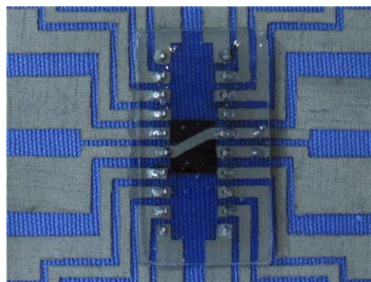
Fig. 3 Solder joints encapsulated in epoxy
