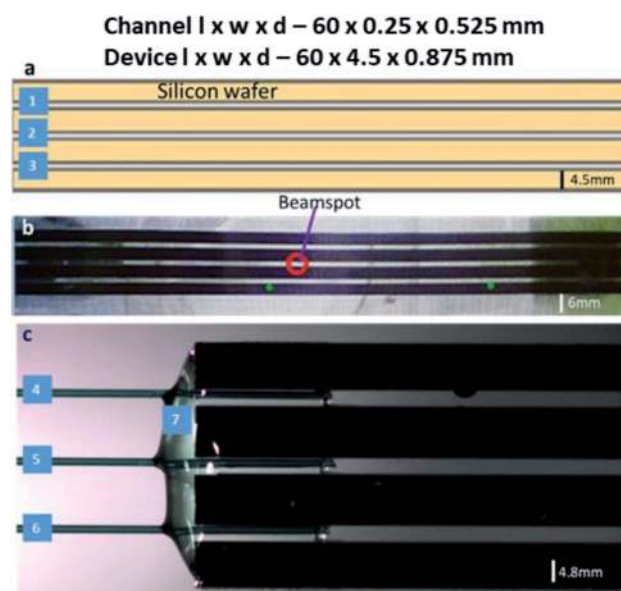
Fig. 3 The microfluidic device and design. (a) CAD diagram of the device with alternate silicon and channel layers (1, 2 & 3); (b) final assembled device mounted on the beamline, a beam of 50 × 50 \mu\text{m}^2 size is focused on the microchannel inside the indicative red circle, which is not the actual beam but indicative of the position; (c) capillaries (4, 5 & 6) glued into the channels using epoxy (7) for flow regulation and connection of PTFE tubing.
