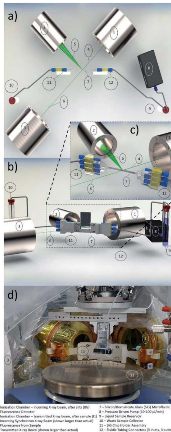
Fig. 2 (a) A schematic view of the XAS microfluidic set up at the beamline; in top view detectors are the ionisation chambers ( I_{0s} before the sample and I_1 after the sample) and the fluorescence detector at 90^\circ angle to the X-ray beam (green line). The microfluidic flow cell (SiG) is positioned at a 45^\circ angle to the beam and fluorescence detector to optimise the signal and with the channel lateral to the table; that can be translated in X, Y and Z. (b) An isometric view of the schematic setup showing the SiG device in position within the chip holder. (c) Close up schematic view showing the SiG chip's orientation within the X-ray beam (chip holder has been removed for clarity, and X-ray beam sizes have been increased for visualisation). (d) Picture from the Balder beamline with the flow cell set up in a glove bag with Kapton® foil (low X-ray background signal) "windows" facing detectors (fluorescence, I_{0s} and I_1 ). The SiG chip is mounted in a chip holder hanging from the translation stage assembly in the beam path as depicted in schematic (a) & (b). Note: all component number labels are given at the bottom of the figure.
