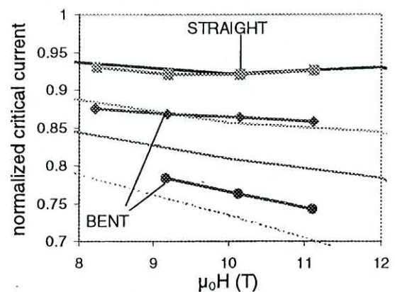
Fig. 7. Normalized Critical Current of 0.7 mm strand cables (A5) reacted straight and bent, compared to cabling and bending degradation measurements performed on strands (see Fig. 3 & 4). Upper line: cabling degradation only; 2 nd and 3 rd line from top: cabling plus bending degradation at 0.2% and 0.41% maximum bending strain; bottom line (dashed): bending degradation calculated [8] with max bending of 0.4%.
