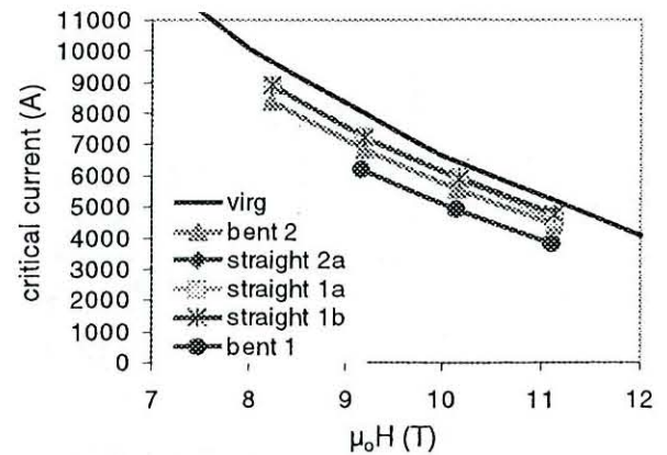
Fig. 6. Critical currents of samples of cables A5 (here with a on virgin strand measurement extrapolated to the cable level) for different fields.
