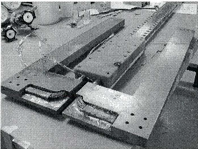
Fig. 5. Cable critical current sample-holder before insertion into test-station.
