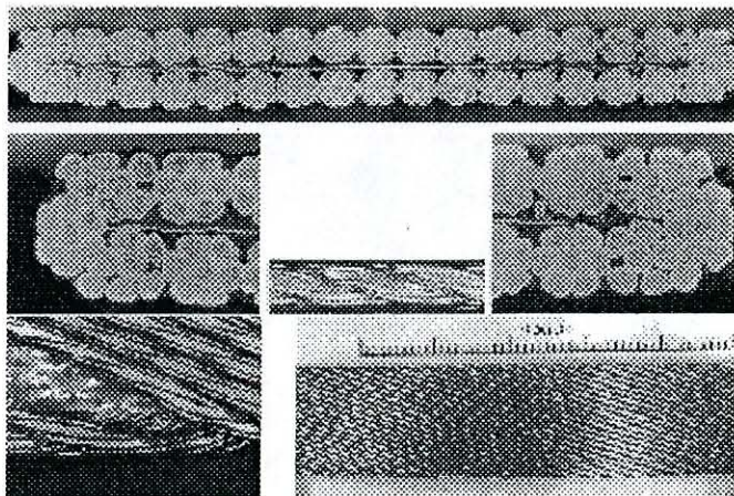
Fig. 1. 0.3 mm strand cable made from 37, 6-around-1, sub-elements.
