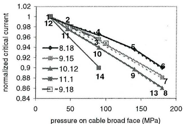
Fig. 8. Effect of transverse pressure on critical current (here normalized on its value at 20 MPa) for different fields. Sample A5 – with bending strain (full symbols), without bending degradation (open symbols). Dashed lines are calculated with Ekin's model.
