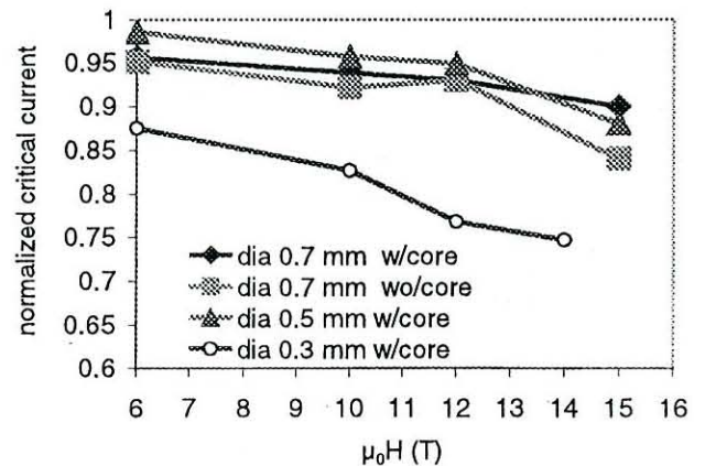
Fig. 3. Cabling degradation measurements on 0.3, 0.5 & 0.7 mm strands.
