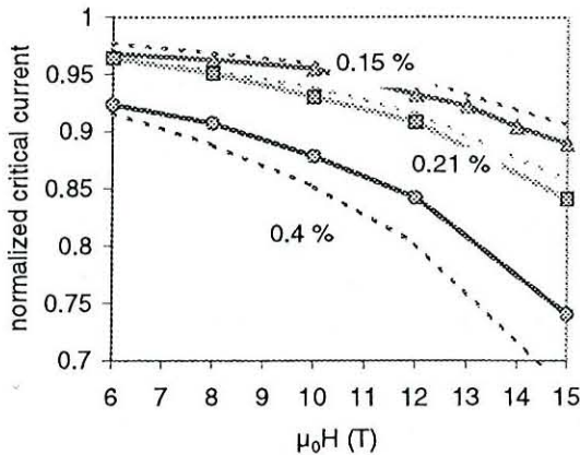
Fig. 4. Degradation of 1 mm (triangles) and 0.7 mm (squares & circles) ITER type strands due to a maximum bending strain of 0.15, 0.21 and 0.4%, compared to calculations (dashed) according to Ekin's deviatorary strain model, assuming an intrinsic filament pre-compression of 0.2%.
