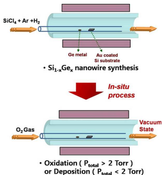
Fig. 1 Schematic of the \text{Si}_{1-x}\text{Ge}_x heterostructure nanowires synthesized procedure. After the growth of \text{Si}_{1-x}\text{Ge}_x nanowires, the flow of \text{SiCl}_4 was terminated and then a flow of \text{O}_2 was introduced under vacuum maintained by mechanical pump
