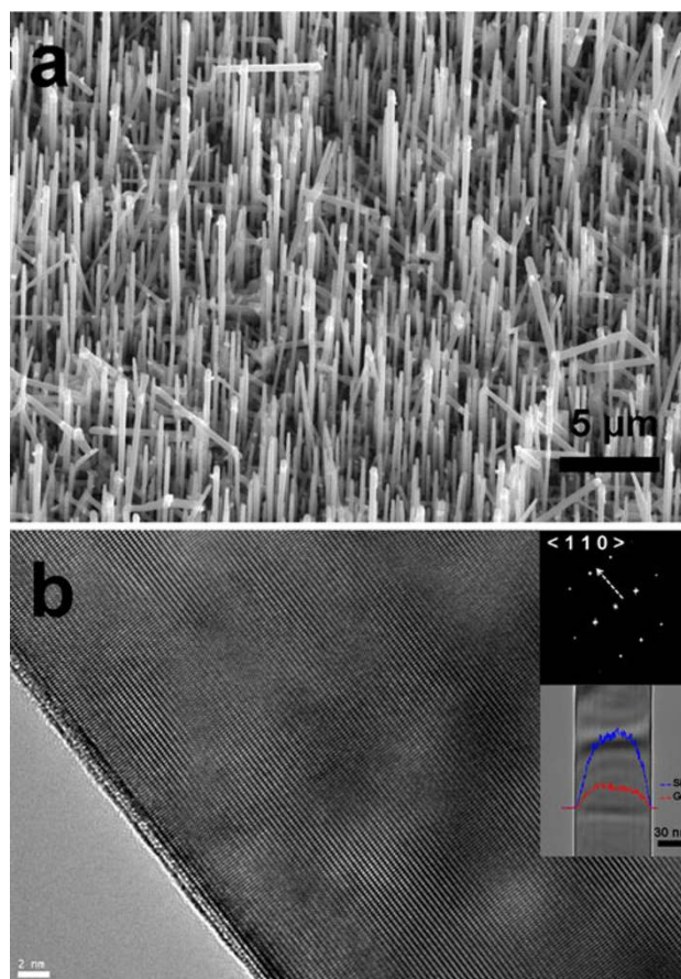
Fig. 2 a SEM image of \text{Si}_{1-x}\text{Ge}_x nanowires with diameter ranged from 50 to 300 nm. b TEM image of individual single crystal \text{Si}_{1-x}\text{Ge}_x nanowires with a thin layer of native oxides. Upper inset is SAED pattern image that shows the nanowire is single crystal and a growth direction is \langle 110 \rangle . Below inset is EDS profile in the radial direction of the nanowire
