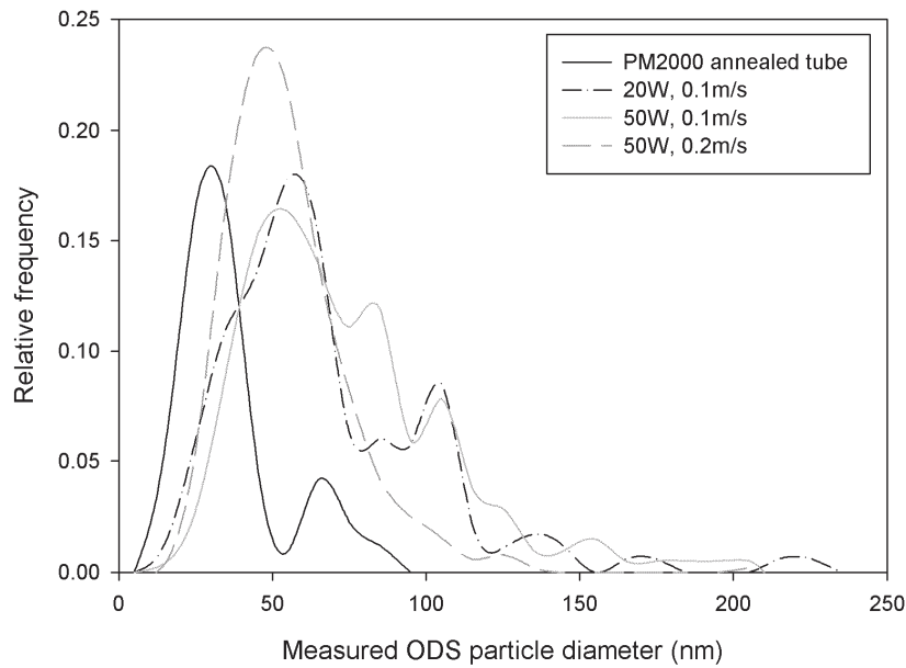
Fig. 6. ODS particle size distribution in PM2000 SLM walls, compared to a conventionally processed PM2000 tube, annealed at 1380°C for 60 minutes.
