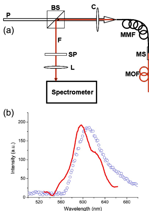
FIG. 4. (Color online) Experimental setup for optical measurement (a), P , pump; BS, beam splitter; C , collimator; MMF, multimode fiber; MS, mechanical splicer; F , fluorescence; SP, short-pass filter; L , lens. Detected fluorescence spectra (b) correspond to single-photon (532 nm, open circle) and two-photon (890 nm, solid line) pumping, respectively.
