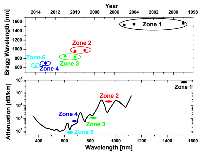
Figure 1. Historical evolution of the operating wavelength of PMMA POF Bragg grating since 1999 as well as the typical attenuation spectrum of PMMA POF.
